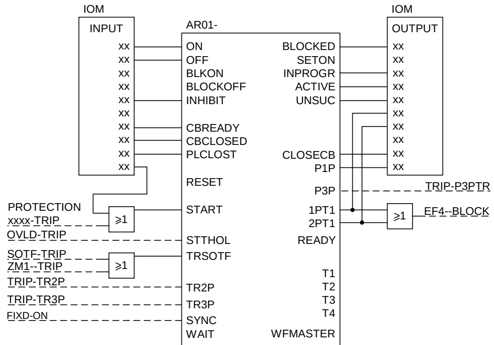
Figure 203: Recommendations for I/O-signal connections
