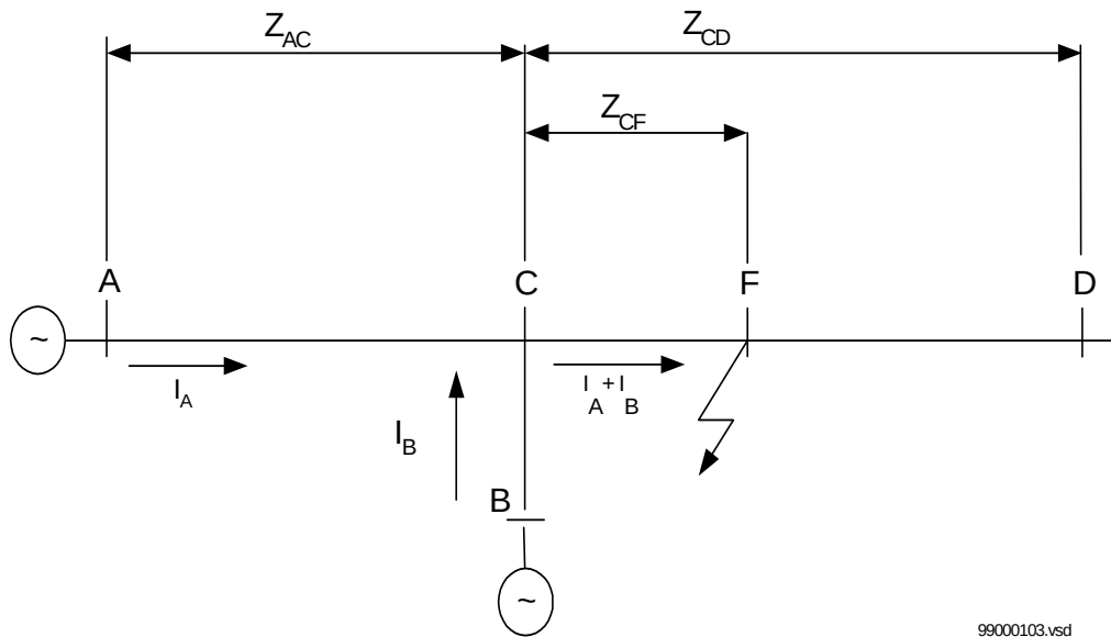
Figure 37: Network with line tied at an intermediate location
