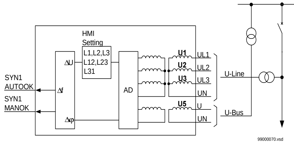
Figure 177: Connection of the synchrocheck function for one bay.
