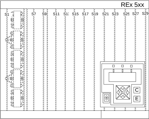
Figure 273: Hardware structure of the 3/4x19" case
