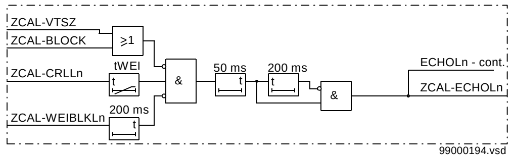
Figure 102: Echo of a received carrier signal by the WEI function.
