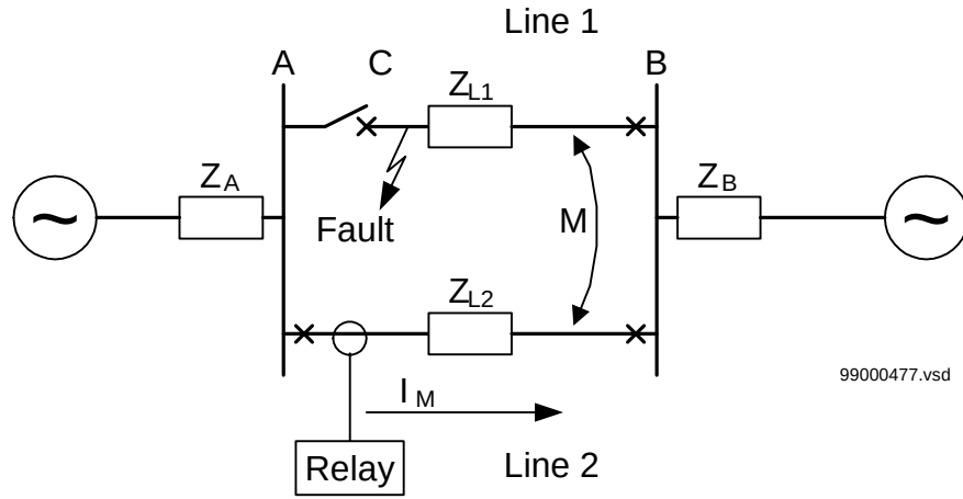
Figure 109: Two parallel lines. Influence from parallel line to the through fault current: I_M
