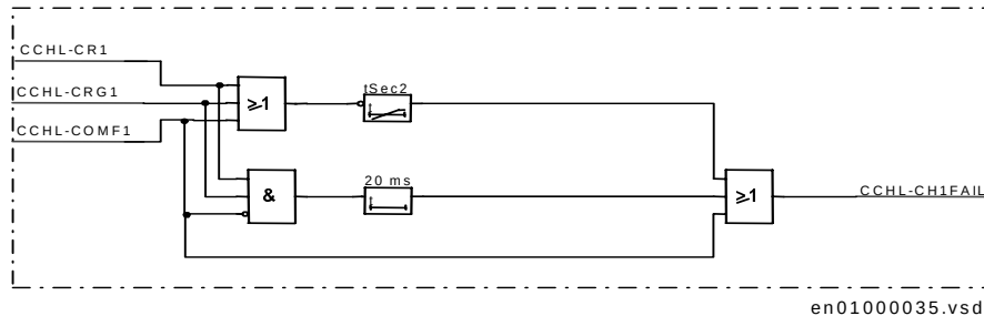
Figure 220: communication channel fail logic.
