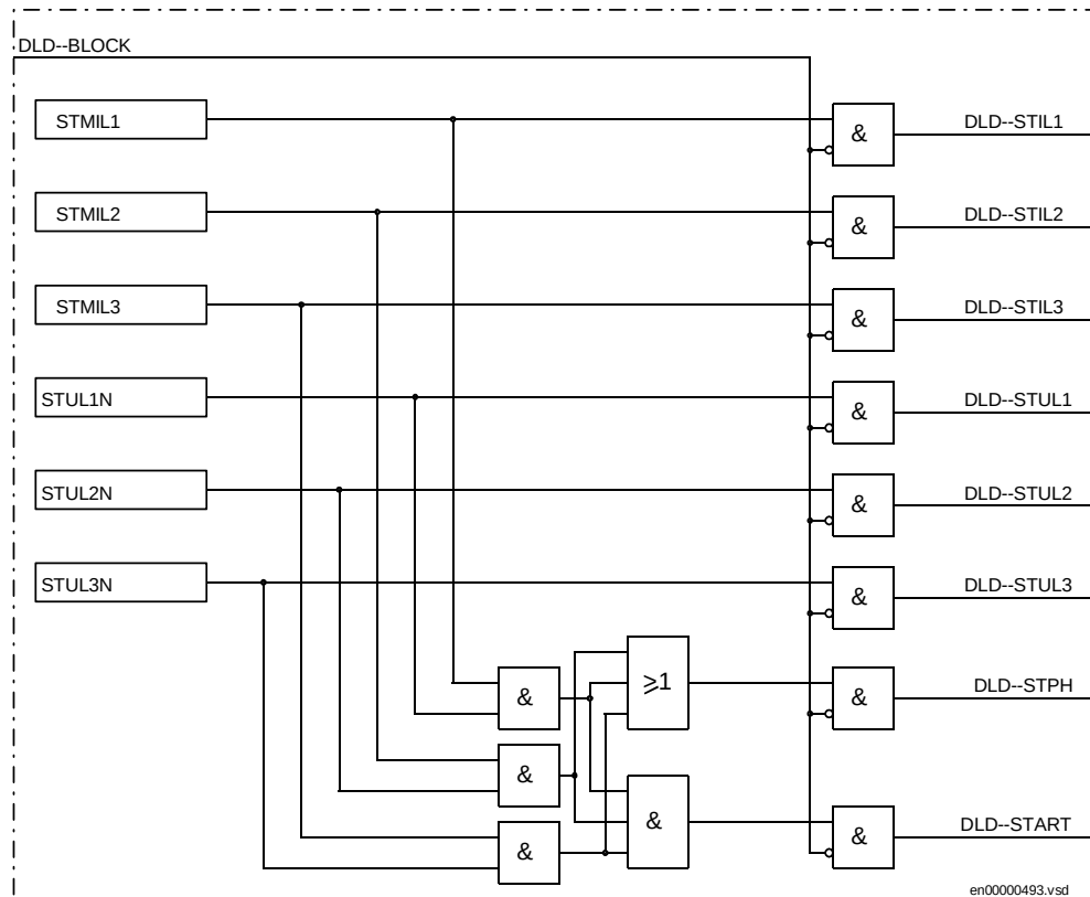
Figure 167: DLD - simplified logic diagram of the dead line detection function
