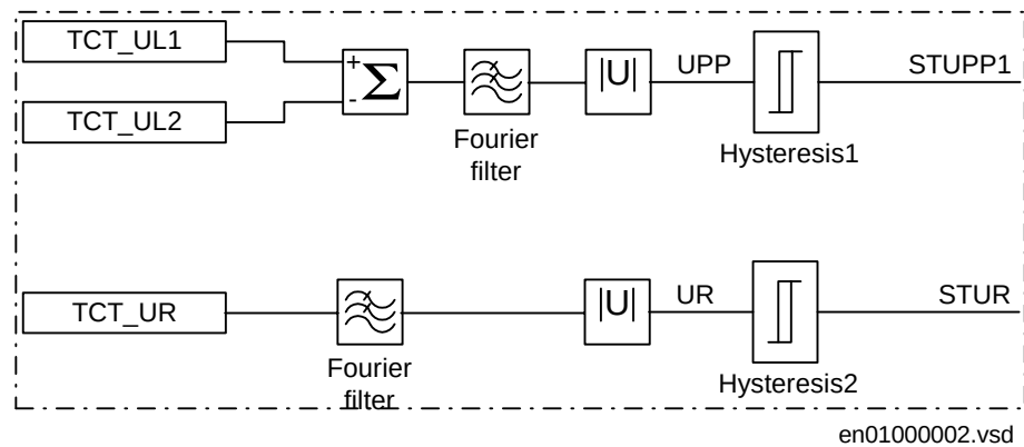
Figure 172: Phase-to-phase voltage and residual voltage measurement
