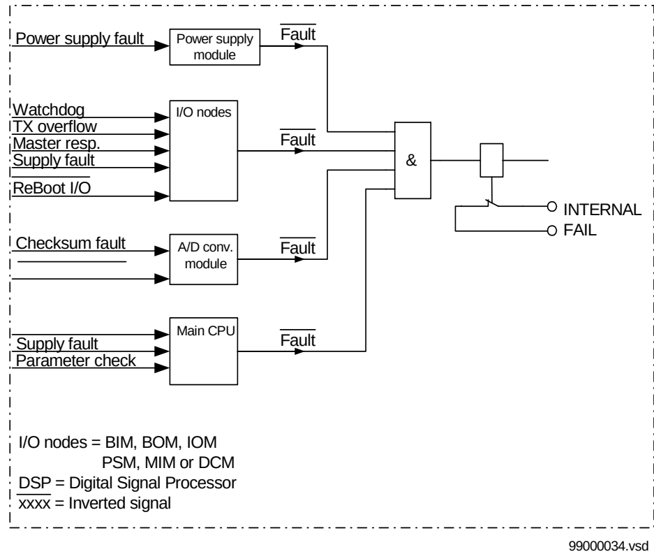
Figure 24: Hardware self-supervision, potential-free alarm contact.
