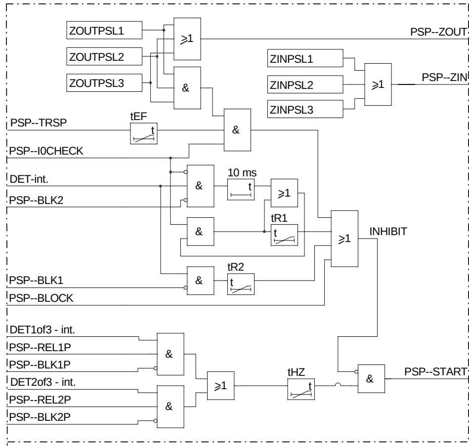
Figure 78: Logic for cooperation with distance protection function.
