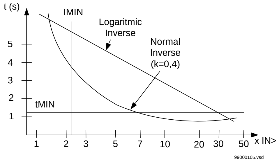
Figure 125: Normal inverse and logarithmic inverse time characteristics.
