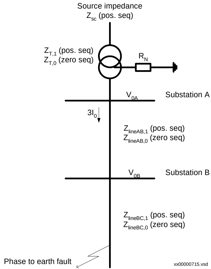
Figure 143: Equivalent of power system for calculation of setting
