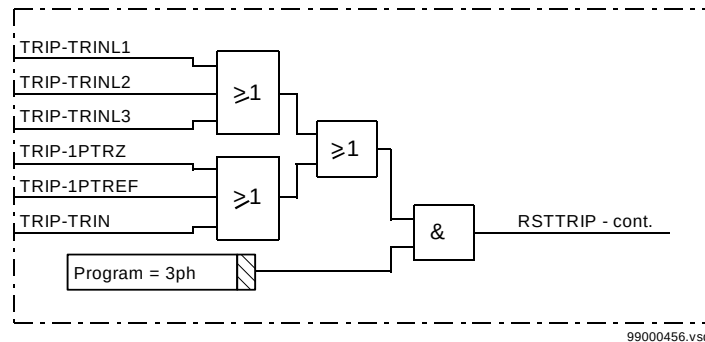
Figure 209: Three-phase front logic - simplified logic diagram
