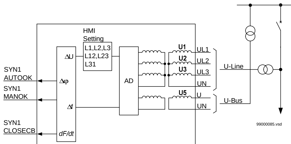
Figure 184: Connection of the phasing and synchrocheck function for one bay.
