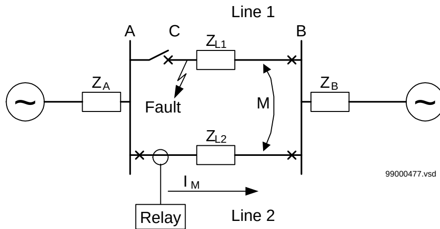
Figure 113: Two parallel lines. Influence from parallel line to the through fault current: I_M .
