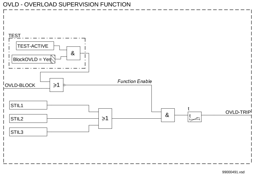
Figure 166: Simplified logic diagram of overload supervision function
