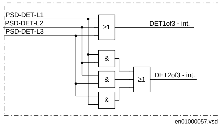
Figure 59: Detection of power-swing for 1-of-3 and 2-of-3 operating mode.
