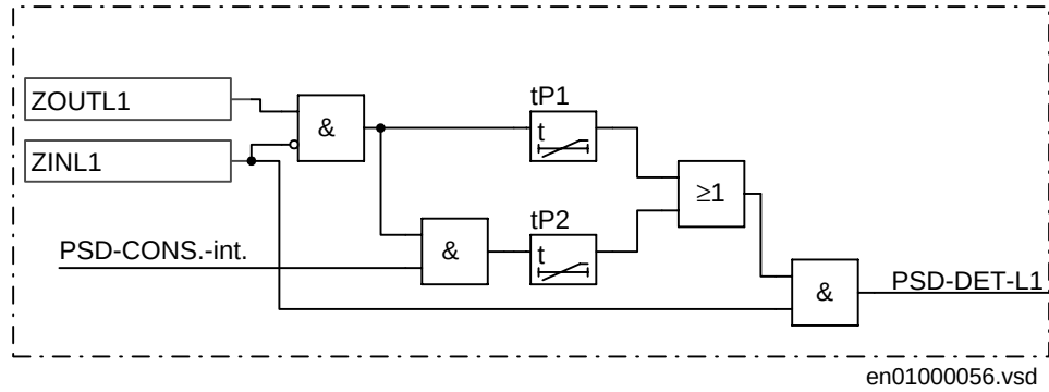
Figure 58: Detection of power-swing in phase L1.
