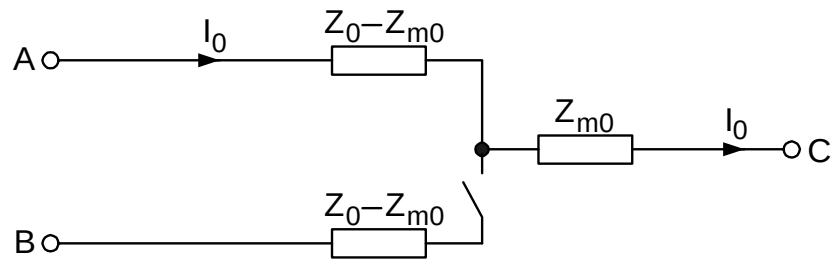
Figure 42: Equivalent zero-sequence impedance circuit for a double-circuit line with one circuit disconnected and not earthed
