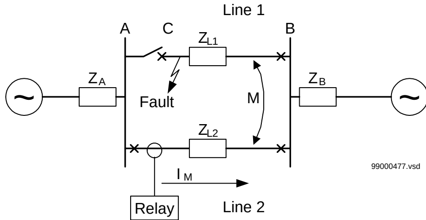
Figure 134: Two parallel lines. Influence from parallel line to the through fault current: I_M
