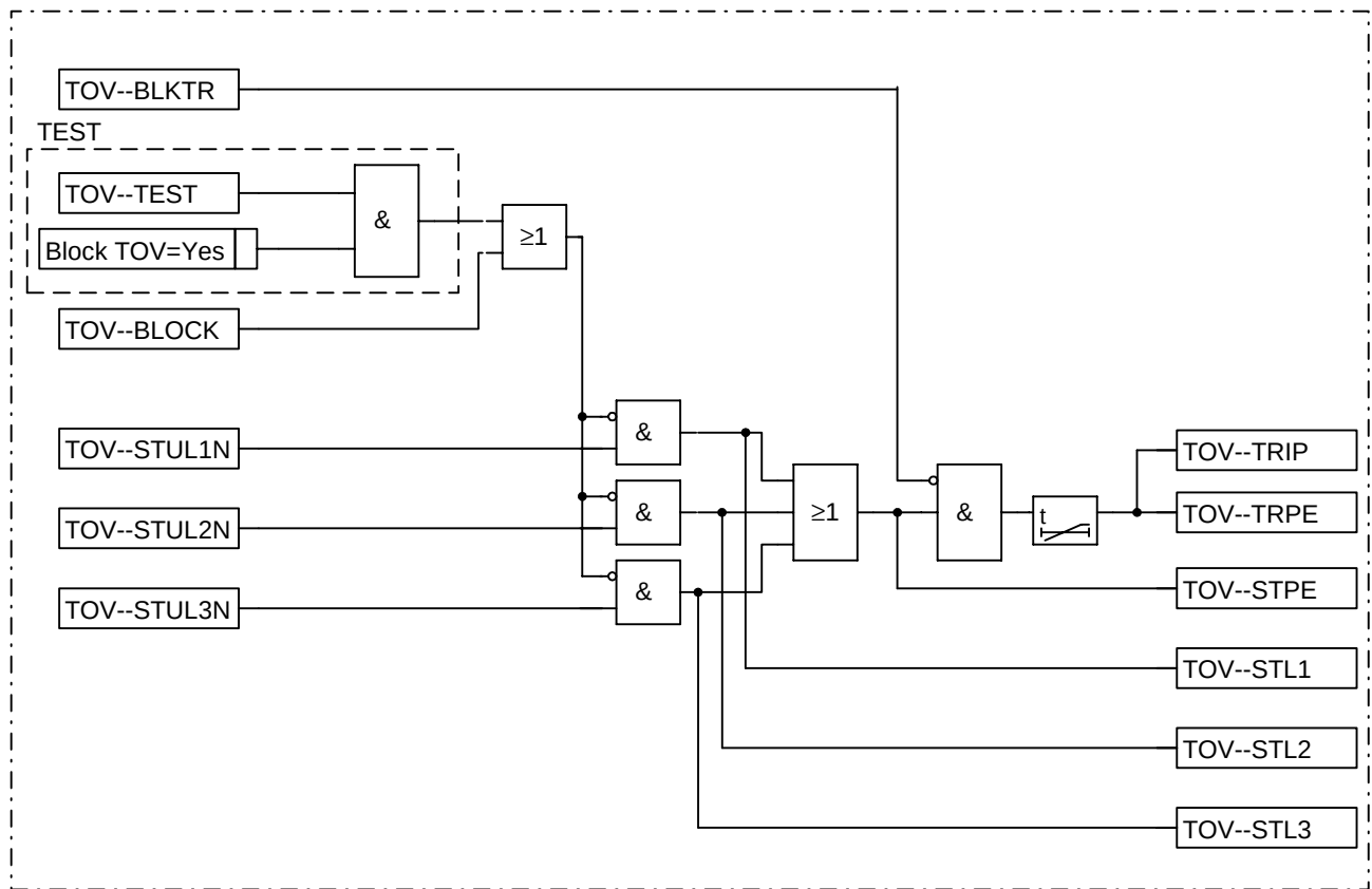
Figure 162: Logic diagram, time delayed overvoltage protection, phase wise
