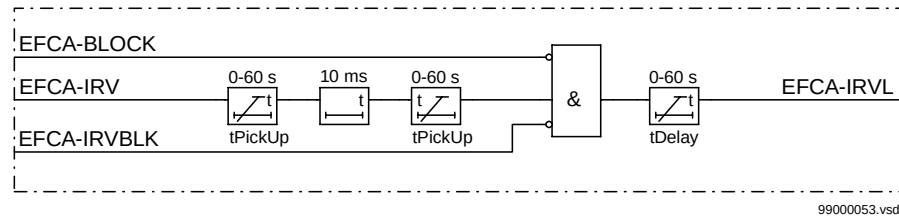
Figure 148: Simplified logic diagram, current reversal
