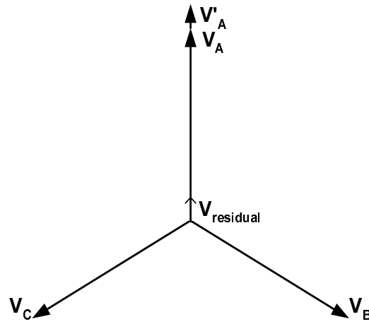
Figure 175: The residual voltage will be equal to the voltage increase in the phase with the broken capacitor element.
