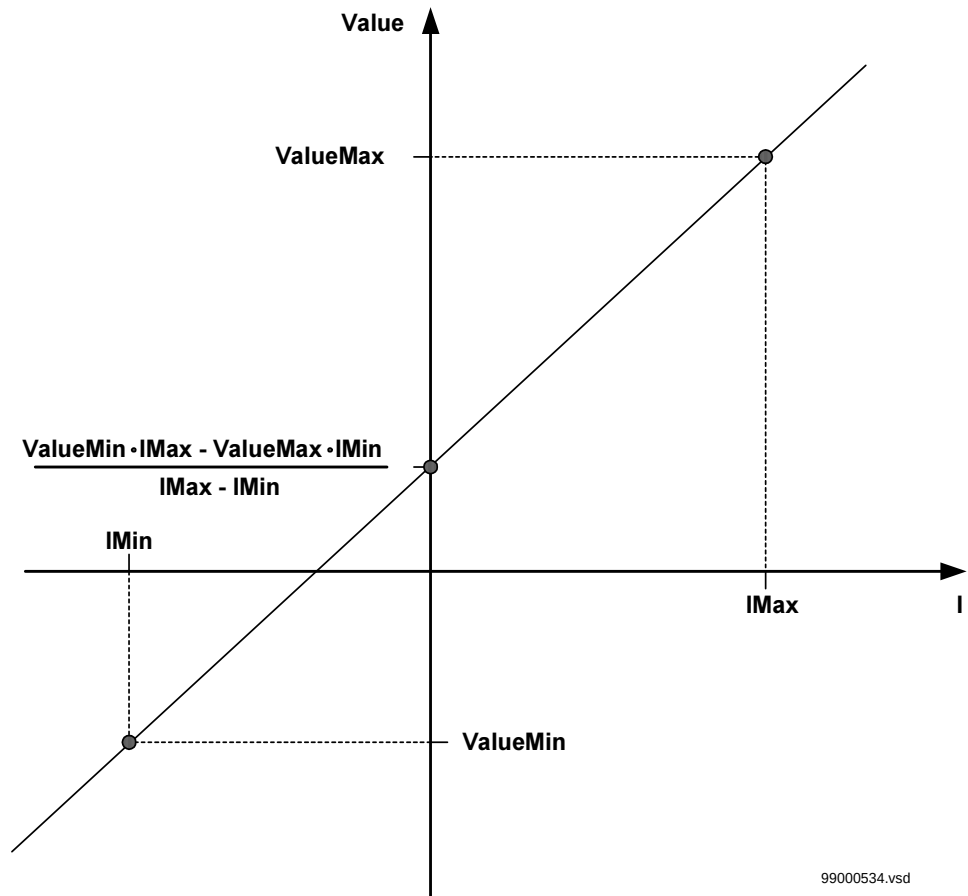
Figure 259: Relationship between the direct current ( I ) and the measured quantity primary value ( Value )
