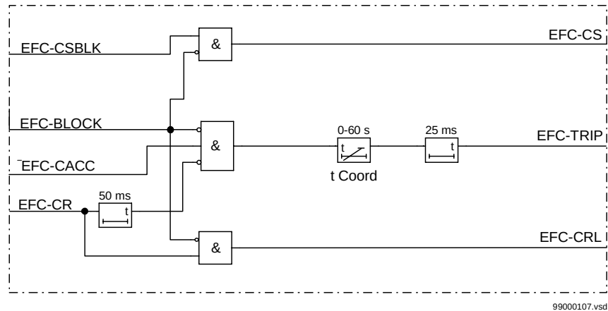
Figure 144: Simplified logic diagram, Scheme type = blocking
