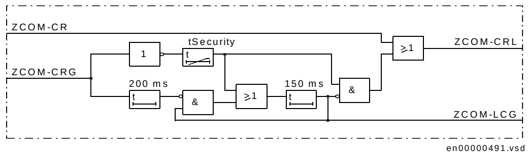
Figure 94: Carrier guard logic with unblock logic.
