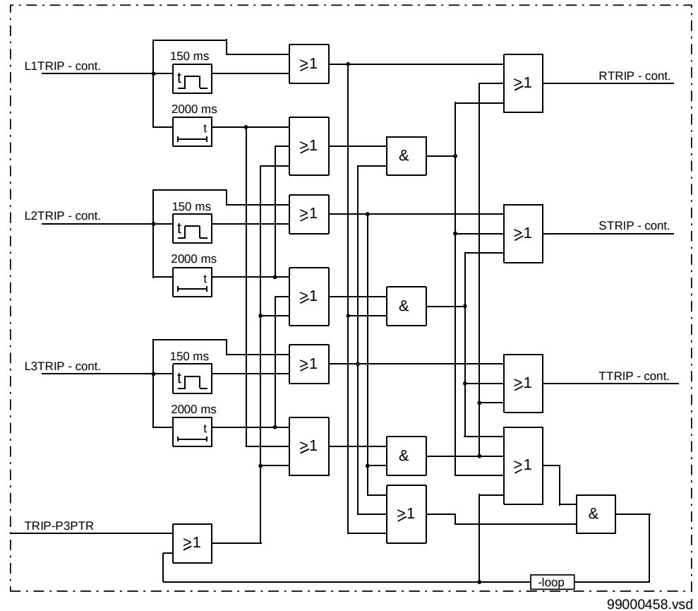
Figure 211: Additional logic for the 1ph/3ph operating mode
