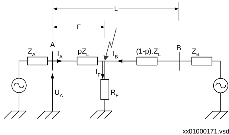
Figure 241: Fault on transmission line fed from both ends.
