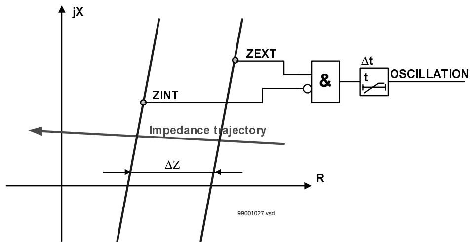
Figure 73: Detection of the oscillation by the (DZ)/(Dt) method.
