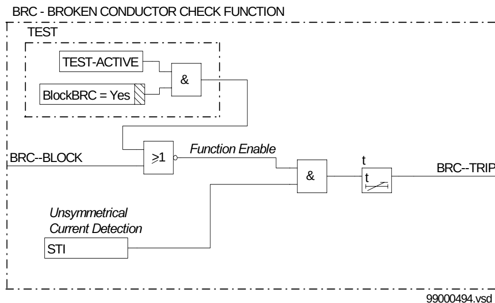
Figure 164: Simplified logic diagram of broken conductor check function
