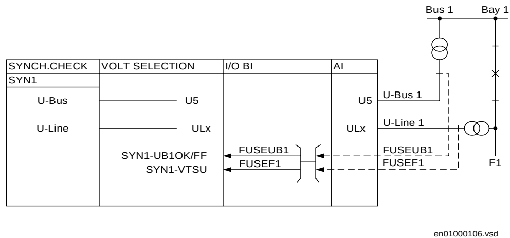
Figure 179: Voltage connection in a single busbar arrangement.
