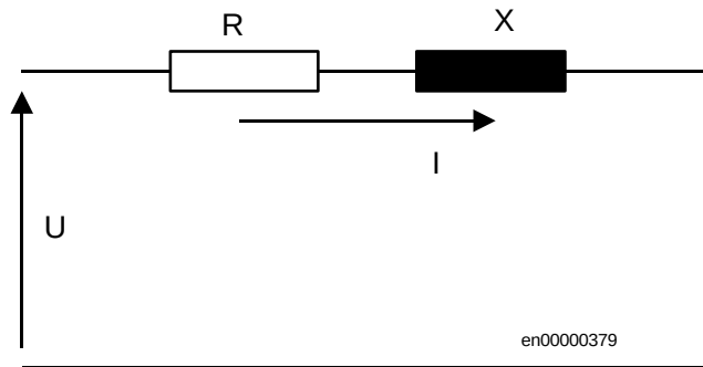
Figure 30: Apparent impedance with resistance and reactance connected in series
