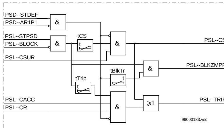
Figure 63: Simplified logic diagram - power swing communication logic.
