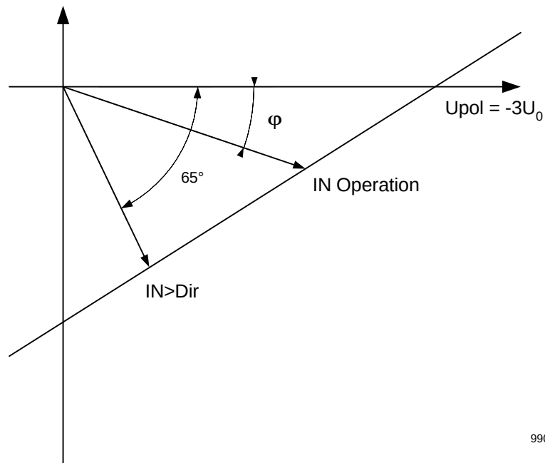
Figure 126: Measuring characteristic of the directional element
