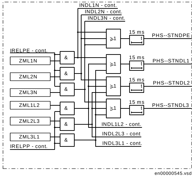
Figure 50: Composition of non directional phase selection signals
