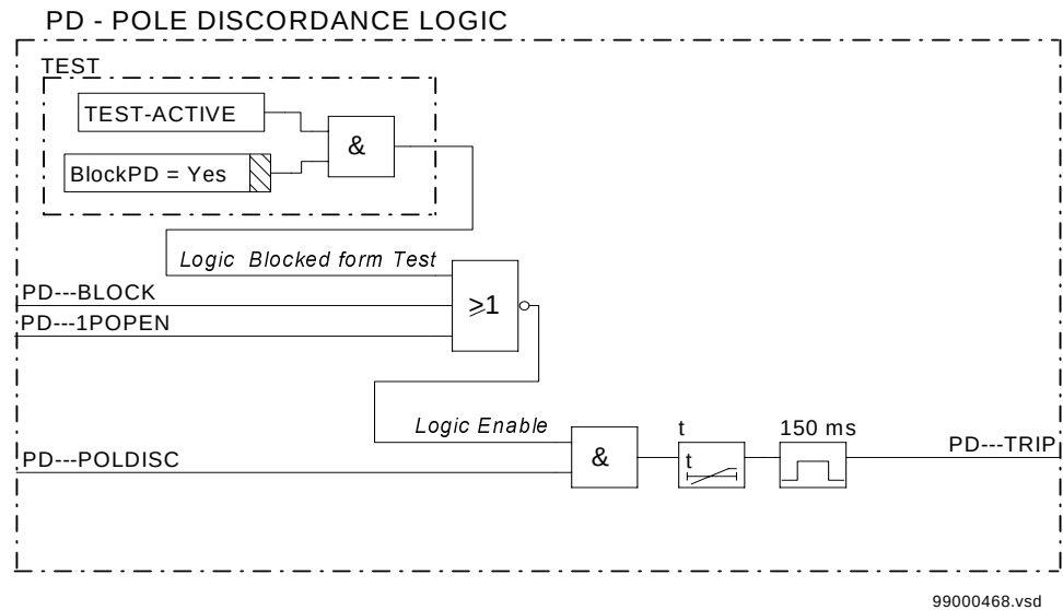
Figure 215: Simplified logic diagram of pole discordance logic - contact based
