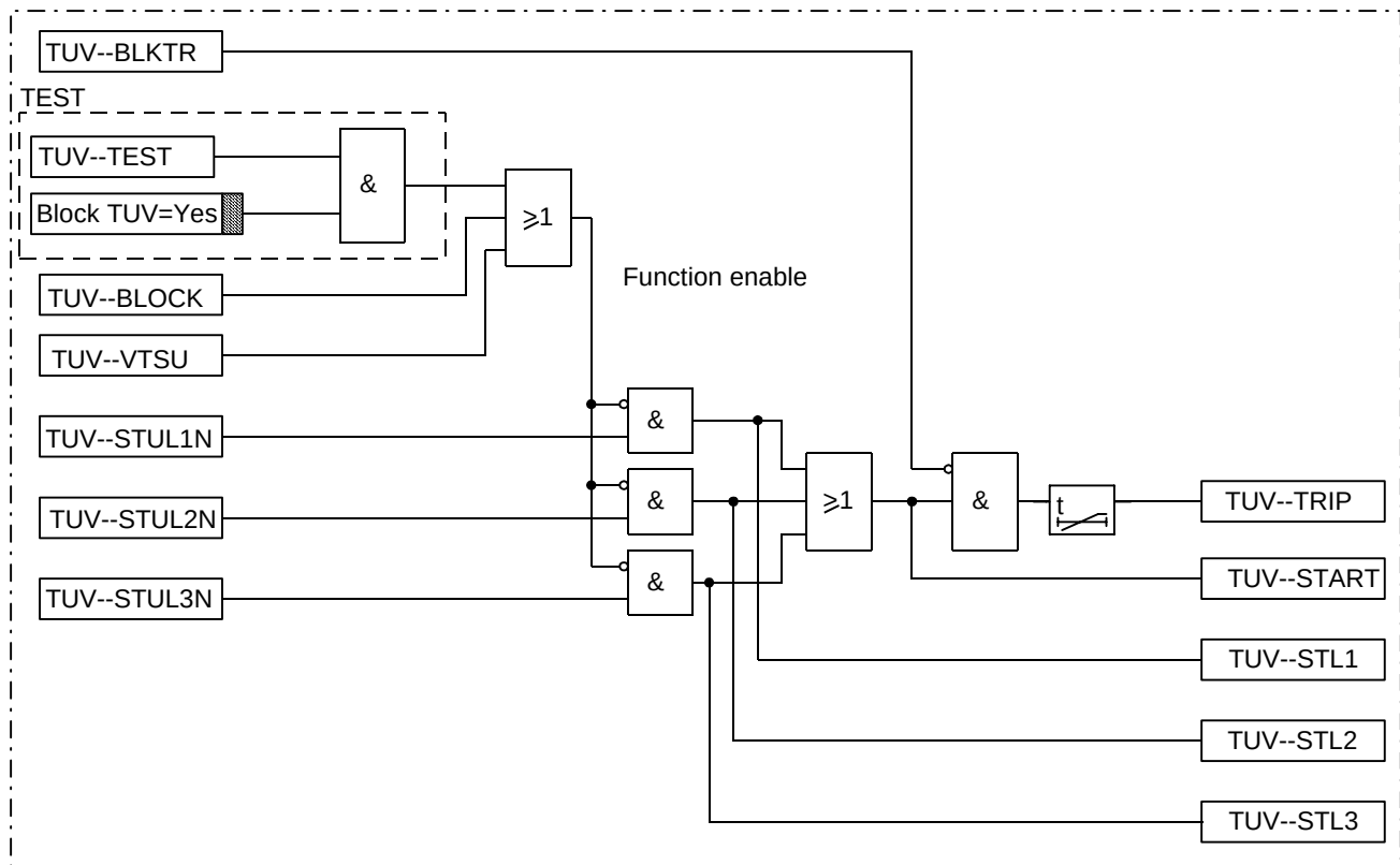
Figure 26: Example of blocking the Time delayed Under-Voltage function.
