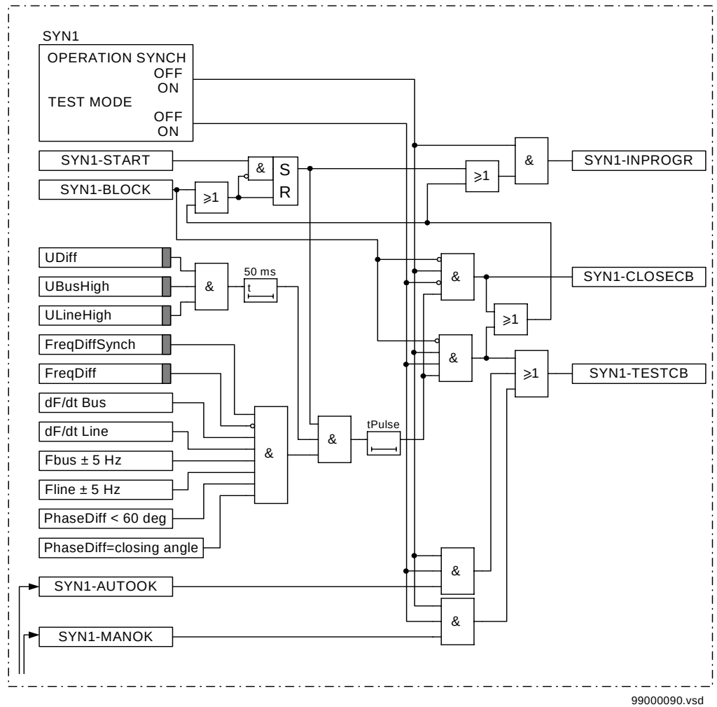
Figure 199: Simplified logic diagram - Phasing. The input signals SYN1-AUTOOK and SYN1-MANOK derive from the synchrocheck and energizing logic.
