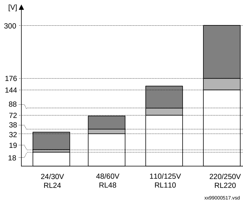
Figure 280: Voltage dependence for the binary inputs
