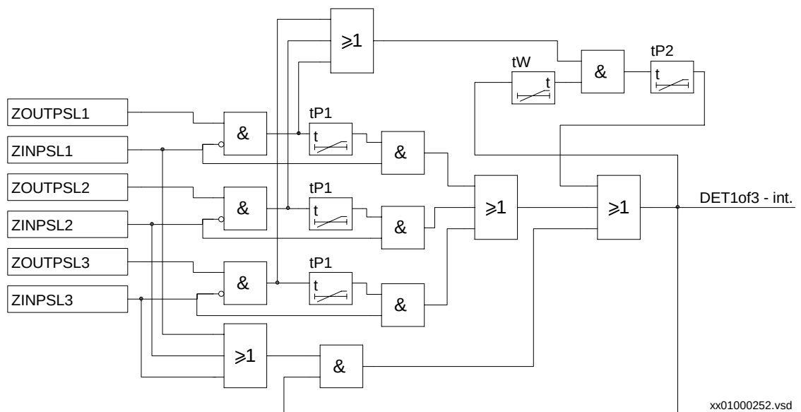
Figure 76: Simplified logic diagram for a one-out-of-three oscillation detection logic
