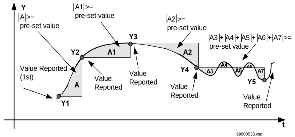
Figure 253: Reporting with integrating dead-band supervision
