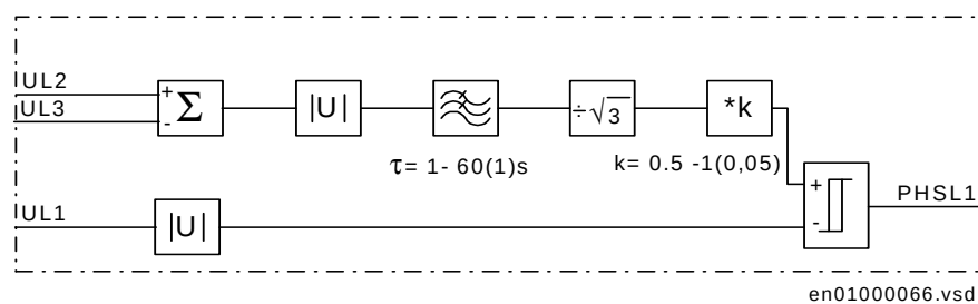
Figure 85: Phase selection function
