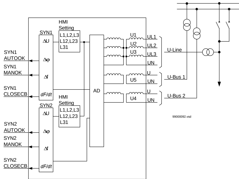
Figure 187: Connection of the phasing and synchrocheck function for one bay.
