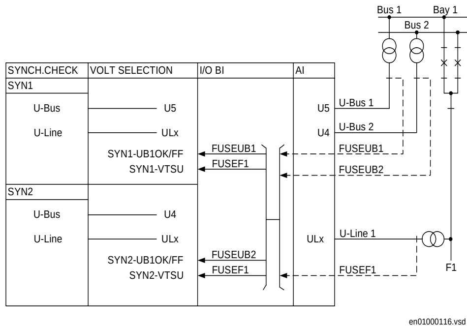
Figure 182: Voltage connection in a double breaker arrangement.
