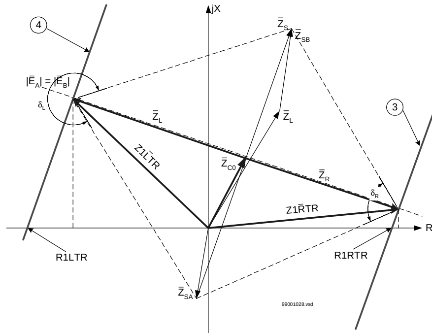
Figure 74: Left (4) and right (3) tripping characteristics and setting of their resistive reach R1LTR and L1RTR respectively.
