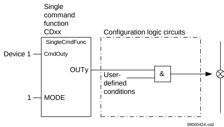
Figure 207: Application example showing a logic diagram for control of external equipment via configuration logic circuits
