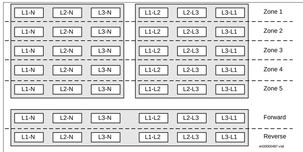
Figure 32: Location of different measuring loops within the three digital signal processors
