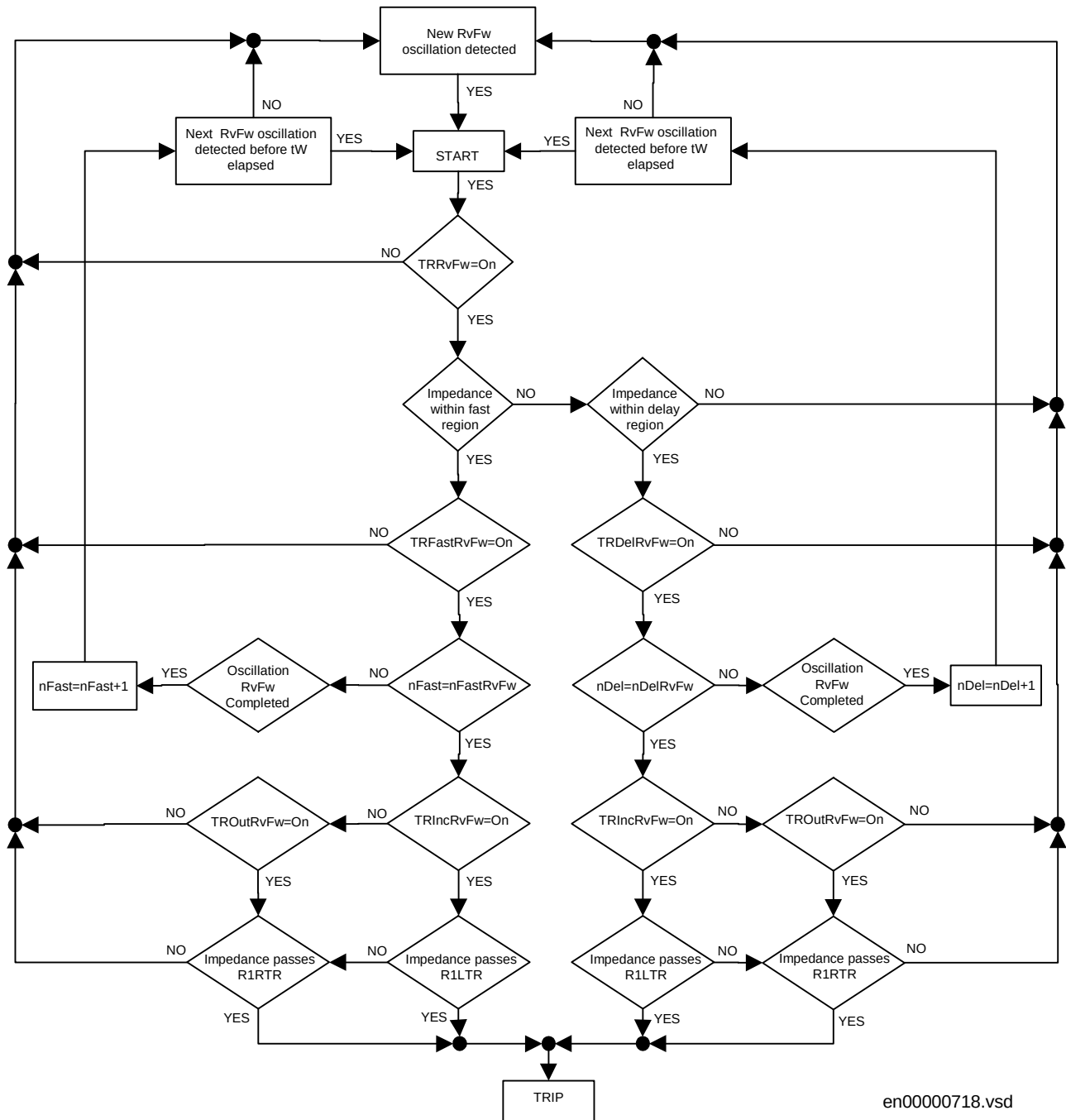
Figure 81: Flow-chart presenting the operation of the pole slip protection for the reverse to forward transition (RvFw) after the oscillation has been detected.
