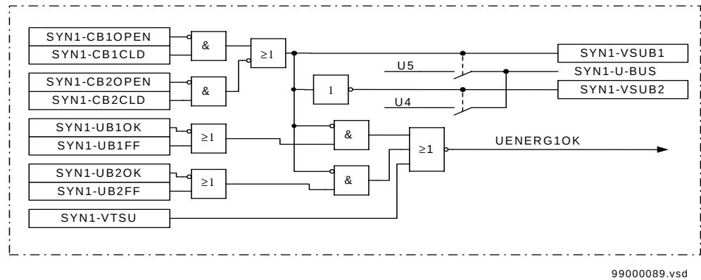
Figure 197: Simplified voltage selection logic in a double bus, single breaker arrangement.
