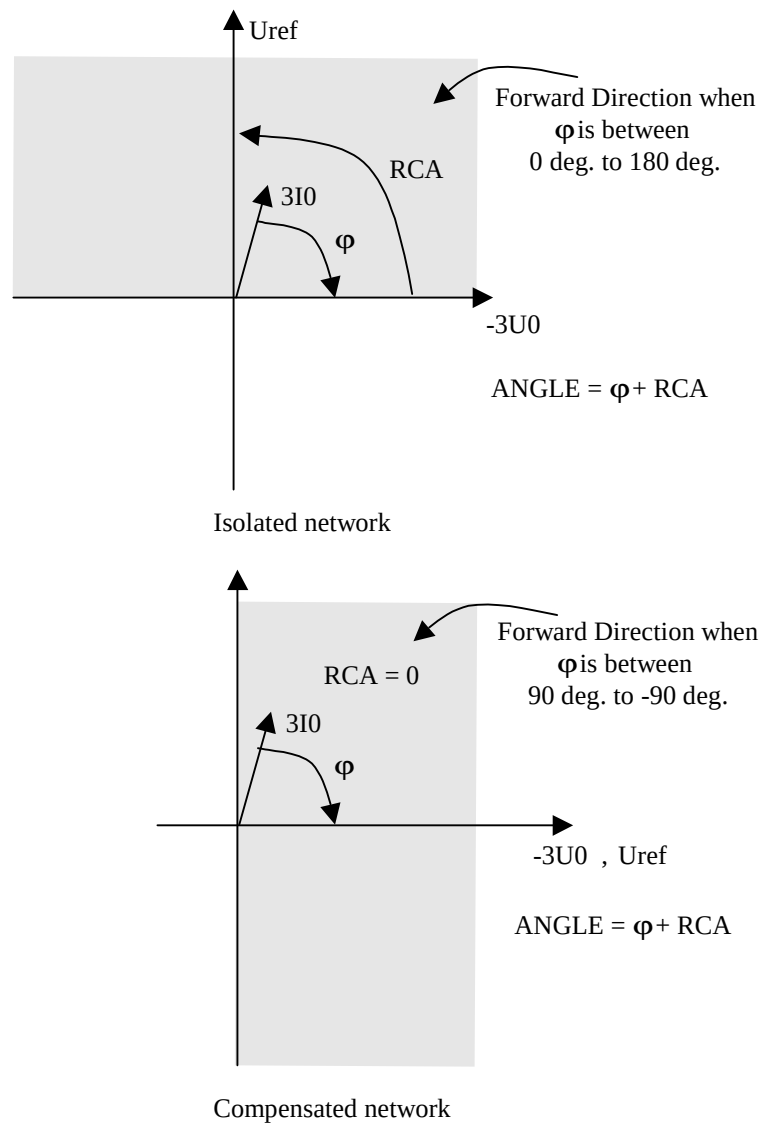
Figure 139: RCA with regard to compensated or isolated network
