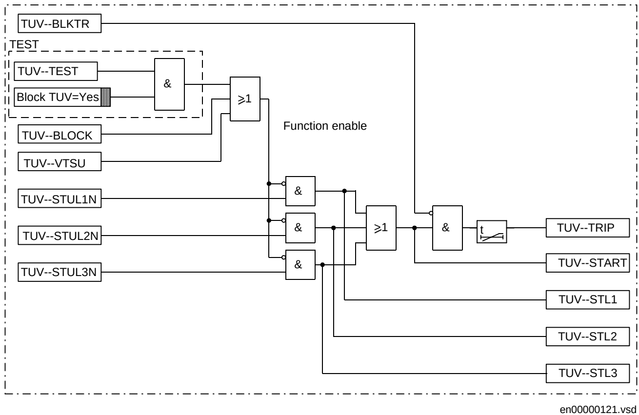
Figure 160: Simplified logic diagram - Undervoltage protection
