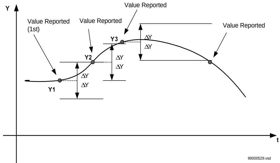
Figure 252: Amplitude dead-band supervision reporting
