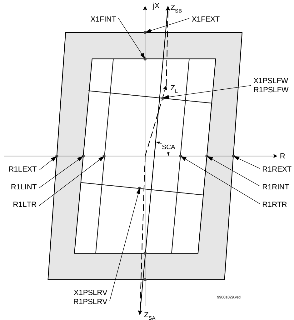
Figure 75: Operating characteristic of the pole slip protection with corresponding settings in the impedance plane.
