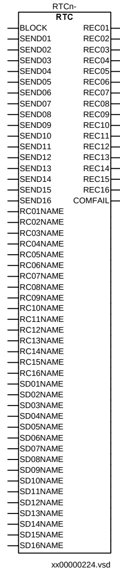
Figure 222: Binary signal transfer to remote end RTC1, signal inputs and outputs
