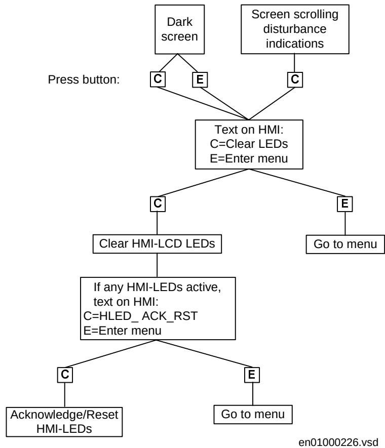
Figure 223: Acknowledgment/reset from local HMI
