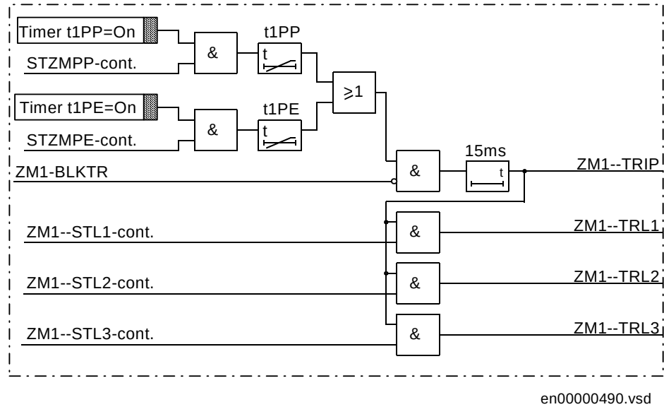
Figure 36: Tripping logic for the distance protection zone one
