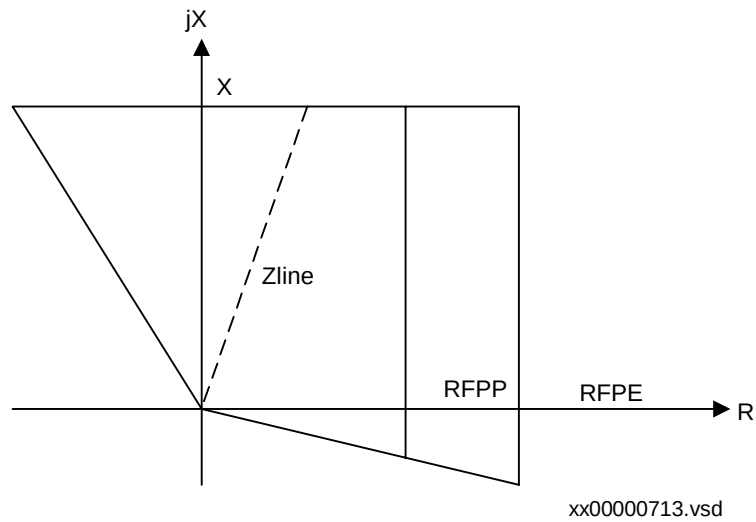
Figure 44: Simplified operating characteristic with R1PP or ( R1PE and R0PE ) or ( R1 and R0 with simplified setting parameters) are set to their minimum values
