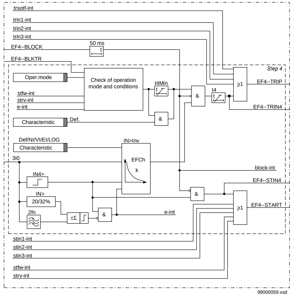
Figure 129: Simplified logic diagram of internal function step 4.
