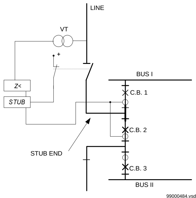
Figure 153: Typical connection for stub protection in 1 1/2 breaker arrangement.
