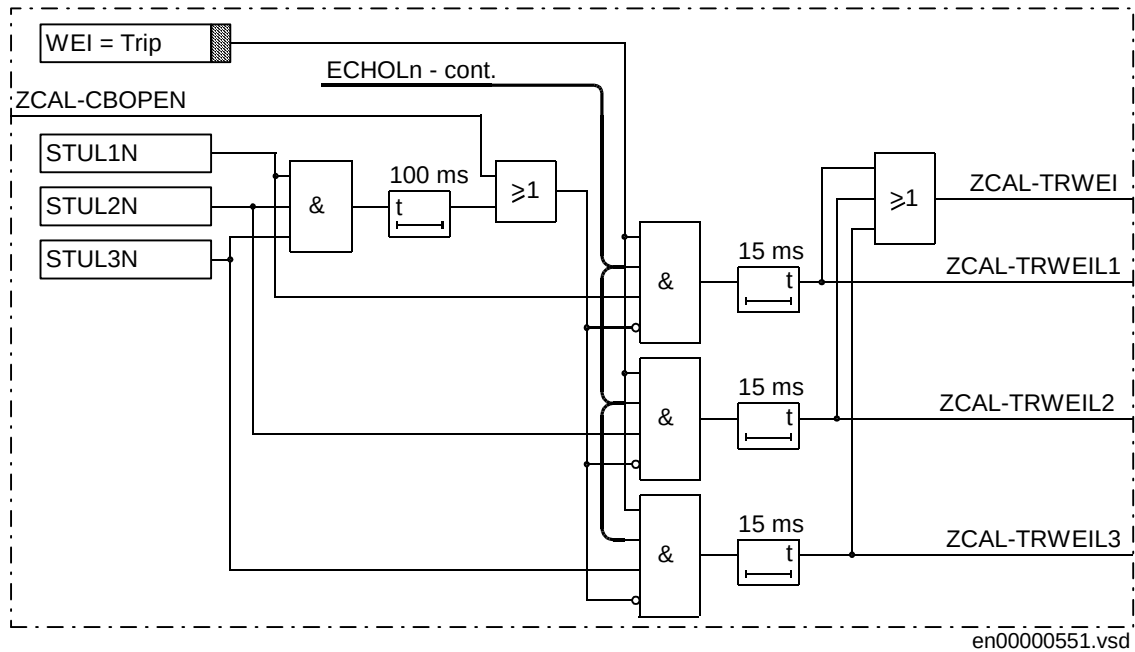
Figure 103: Tripping part of the WEI logic - simplified logic diagram.
