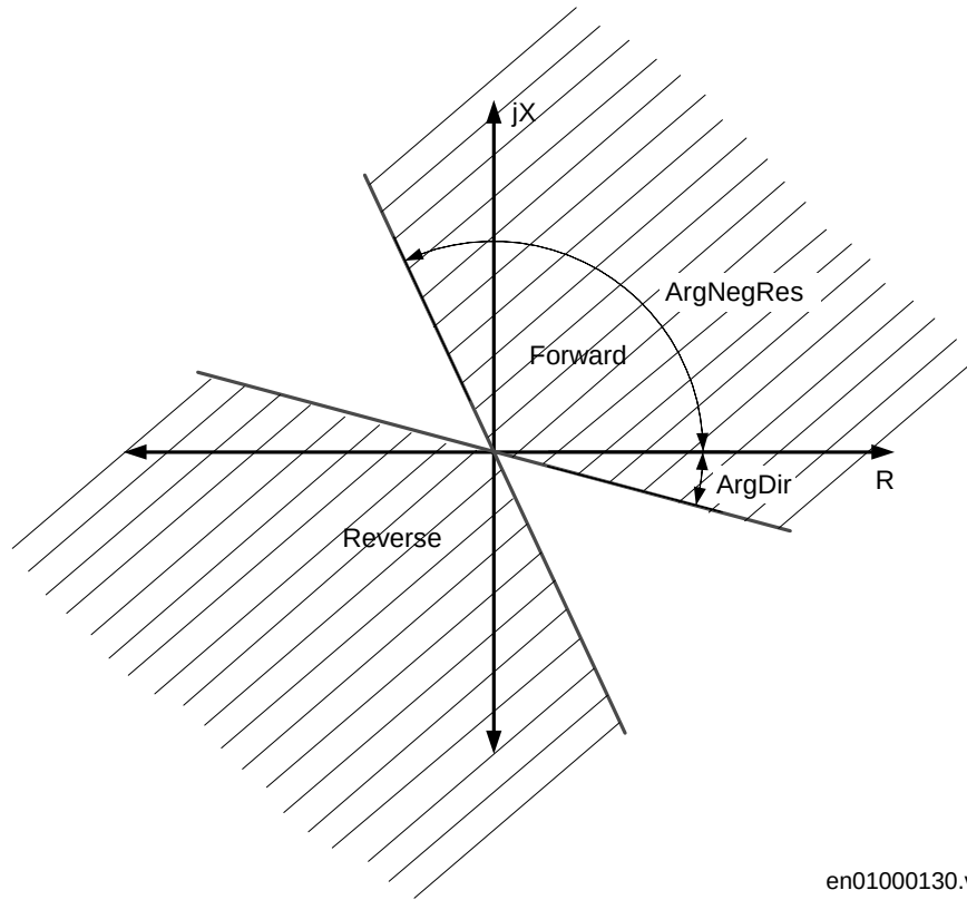
Figure 43: Directional lines define the forward and reverse operating area for each distance protection zone
