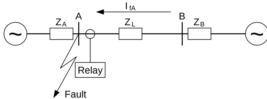
Figure 135: Through fault current from B to A: I_{fA}
