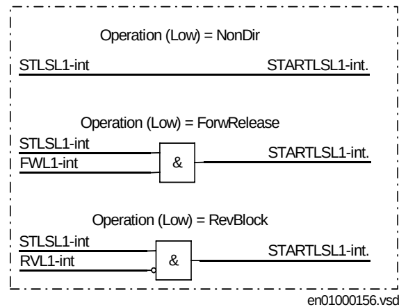
Figure 120: Directional operation modes of TOC3
