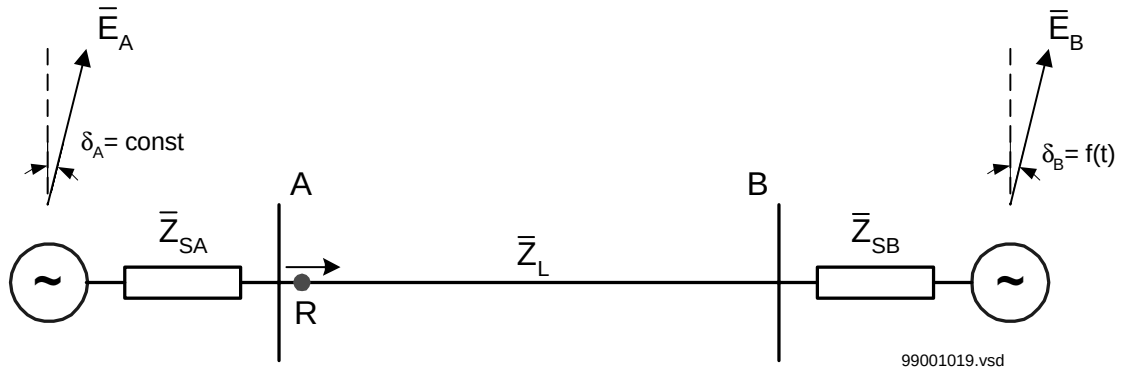
Figure 65: Two machine system.
