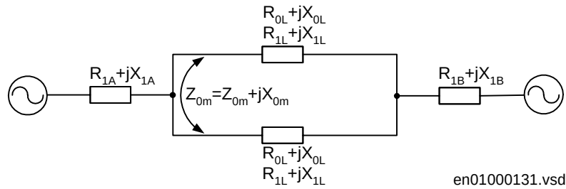
Figure 242: Simplified network configuration with network data, required for settings of the fault location-measuring function.
