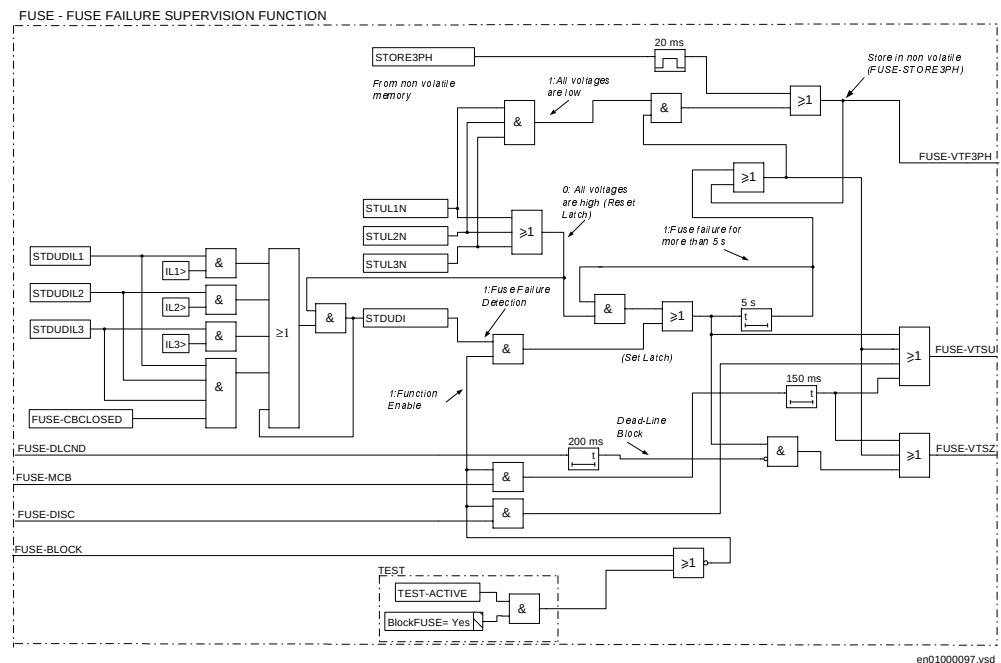
Figure 171: Simplified logic diagram for fuse failure supervision function, du/dt based.
