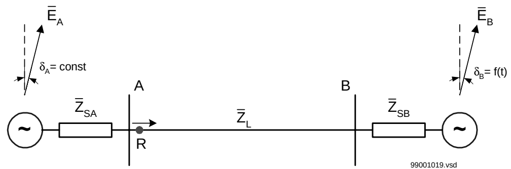
Figure 84: Power system reduced to a two machine system.
