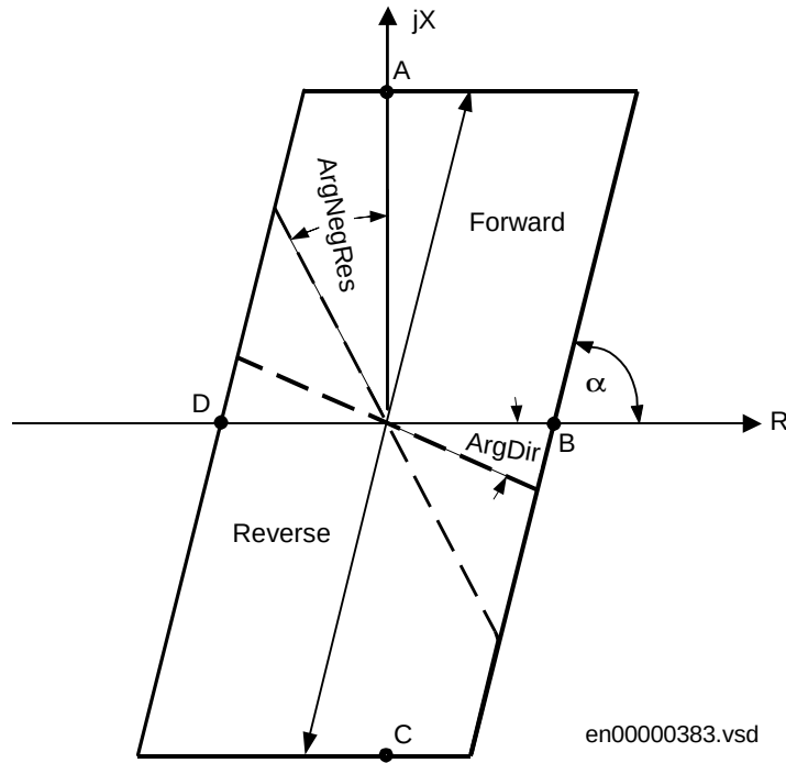
Figure 31: General operating characteristic of impedance measuring elements
