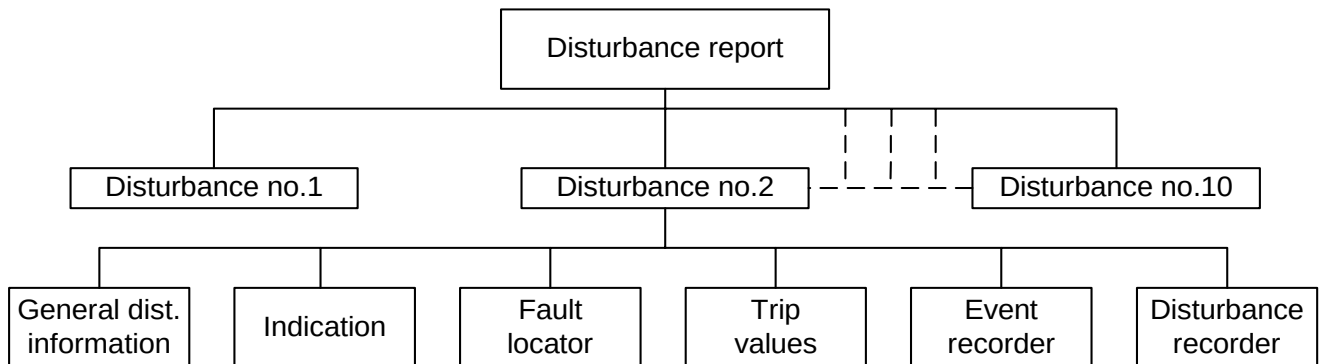
Figure 239: Disturbance report structure
