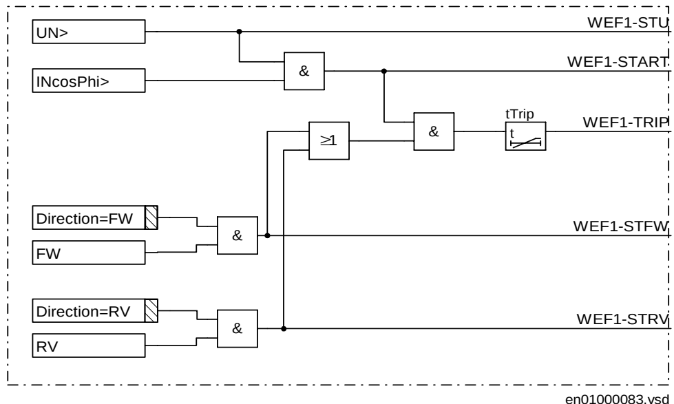
Figure 140: Logic for sensitive directional residual overcurrent protection function (WEF1)
