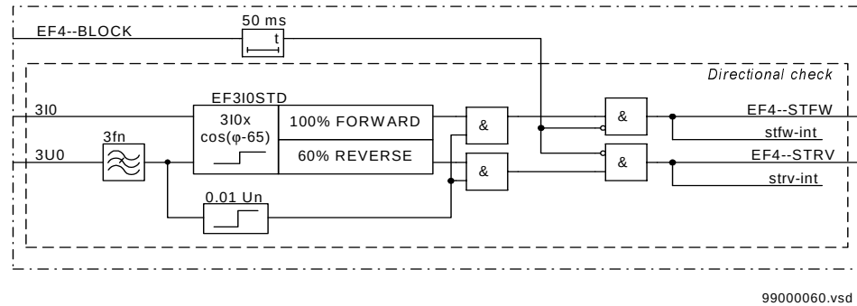
Figure 130: Simplified logic diagram of internal function Directional check.
