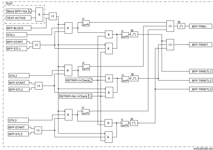
Figure 155: Breaker-failure protection, simplified logic diagram
