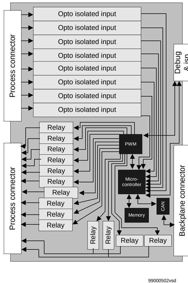
Figure 285: Block diagram for the binary input/output module
