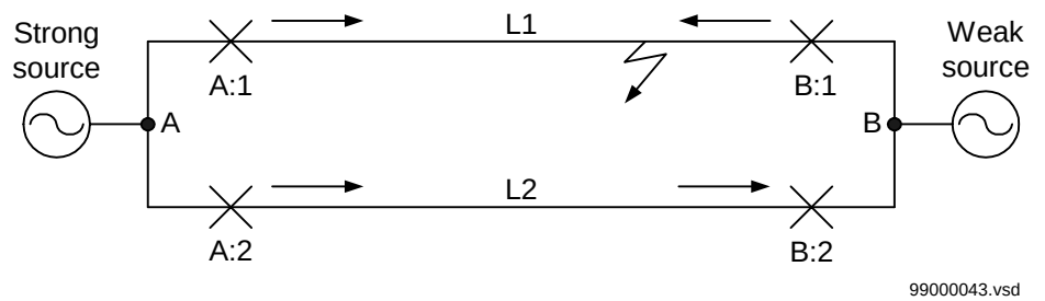
Figure 99: Initial system condition.
