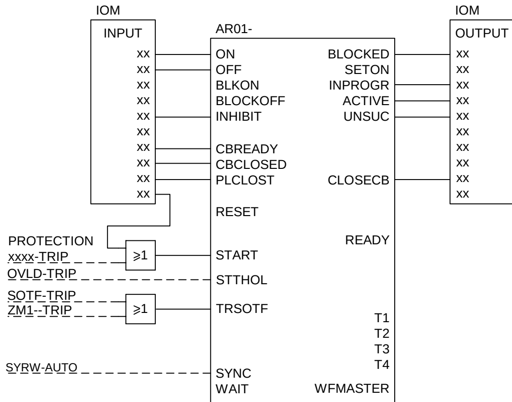
Figure 202: Recommendations for I/O-signal connections
