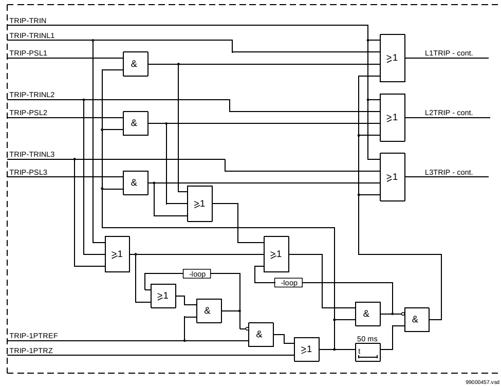
Figure 210: Phase segregated front logic
