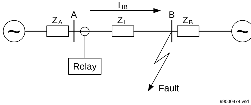
Figure 110: Through fault current from A to B: I_{fB}
