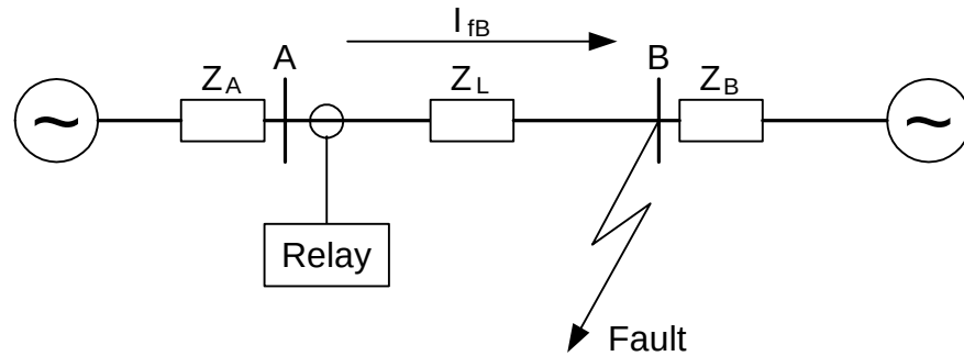
Figure 133: Through fault current from A to B: I_{fB}
