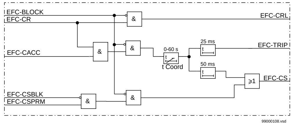
Figure 145: Simplified logic diagram, Scheme type = permissive
