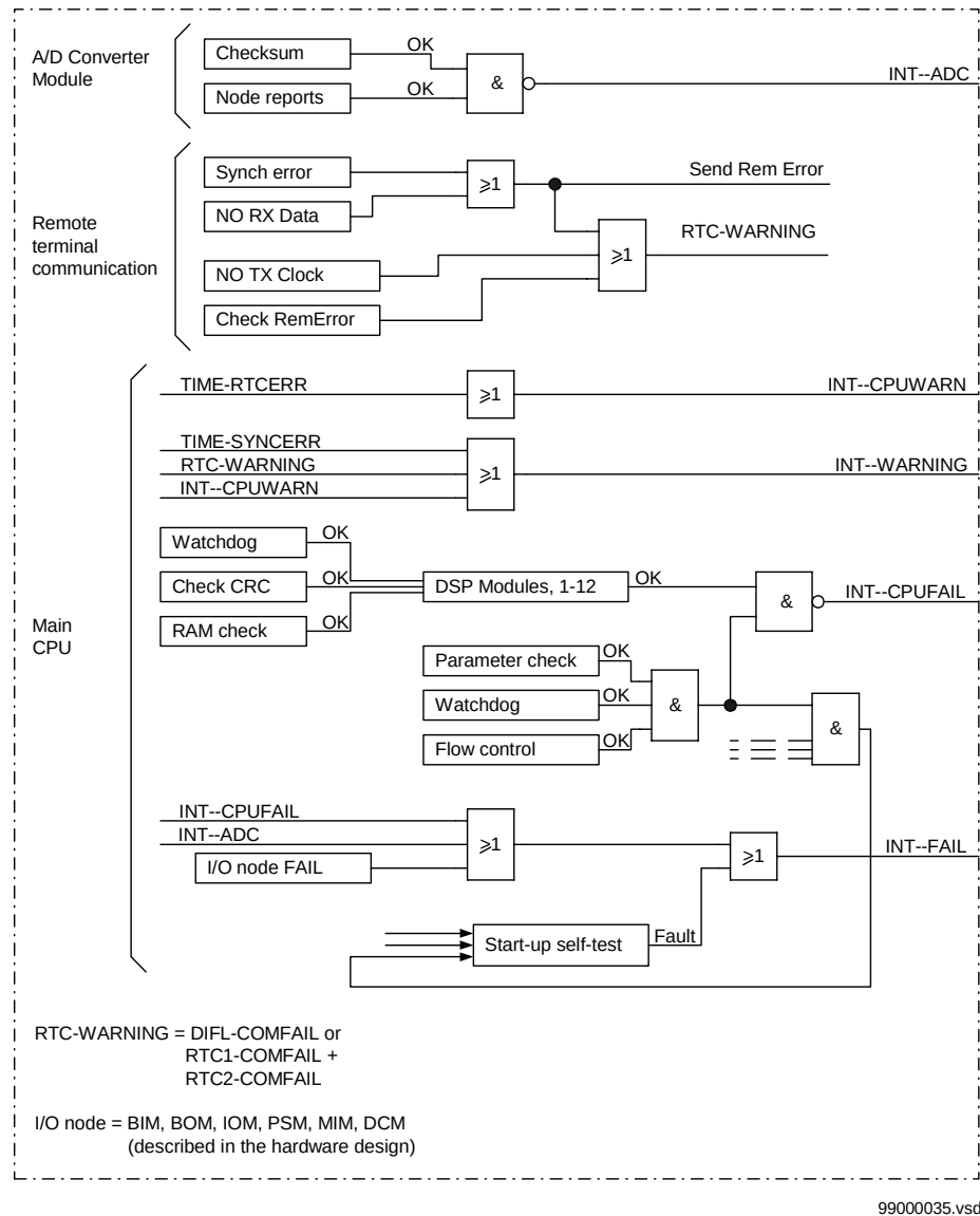
Figure 25: Software self-supervision, function block INTERNAL signals.
