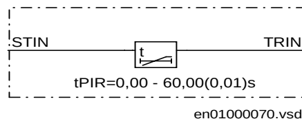
Figure 90: Function for residual current detection
