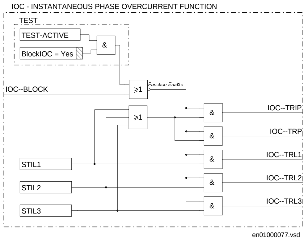
Figure 104: Simplified logic diagram of instantaneous overcurrent protection
