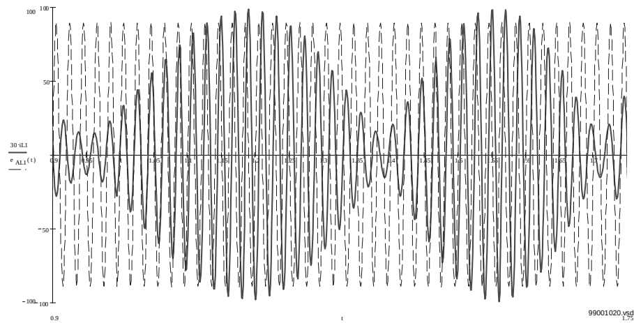
Figure 66: Current (solid line) and voltage (dashed line) in relay point during the pole slip condition.
