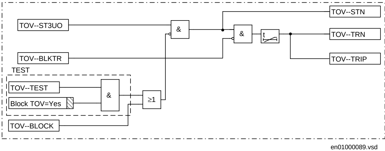
Figure 163: Logic diagram, time delayed overvoltage protection, residual
