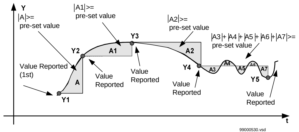
Figure 245: Reporting with integrating dead-band supervision.
