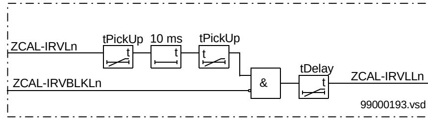
Figure 101: Current reversal logic.
