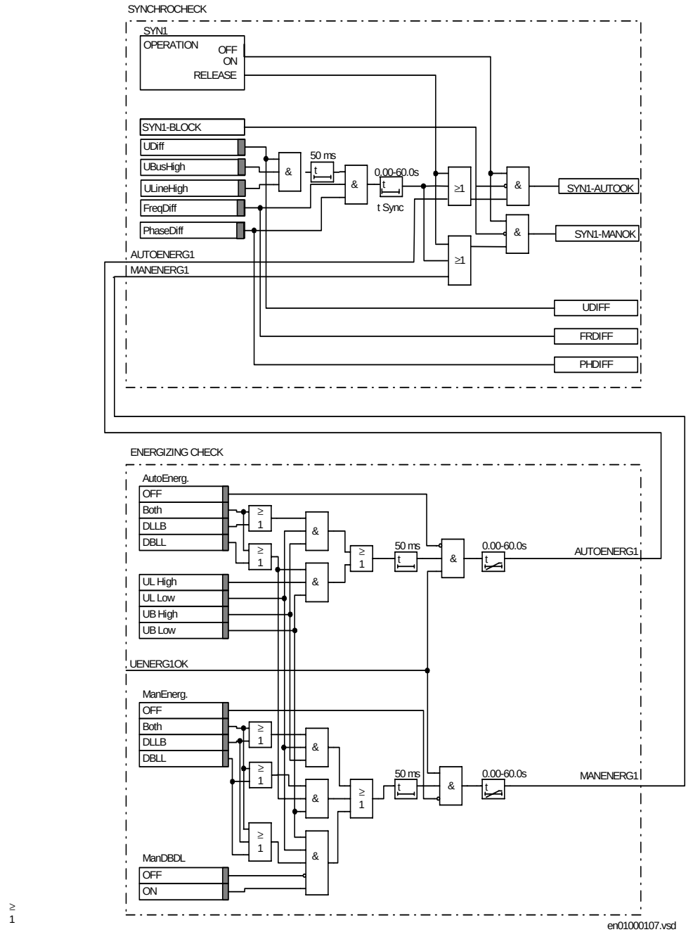
Figure 200: Simplified logic diagram - Synchrocheck and energizing check for one circuit breaker. The internal signal UENERG1OK derives from the external or internal fuse failure inputs SYN1-UB1OK/FF and SYN1-VTSU.
