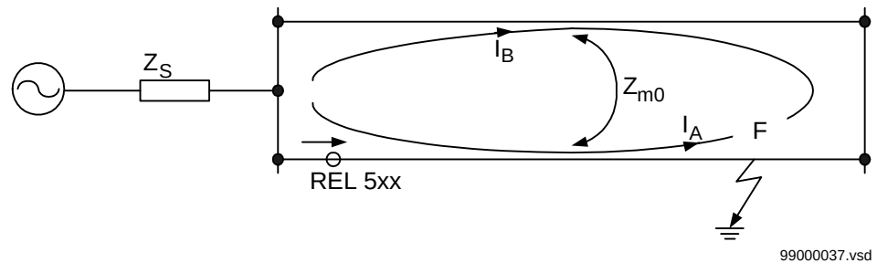
Figure 39: Double-circuit parallel operating line
