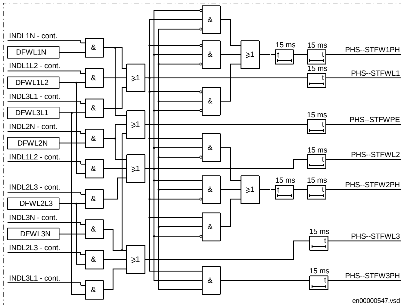
Figure 52: Composition of forward directed phase selection signals
