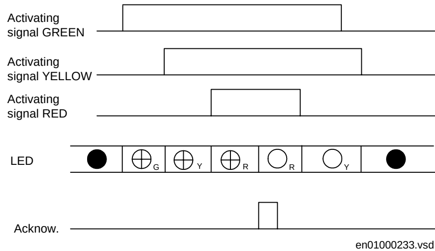
Figure 229: Operating sequence 3, three colors involved, alternative 1
