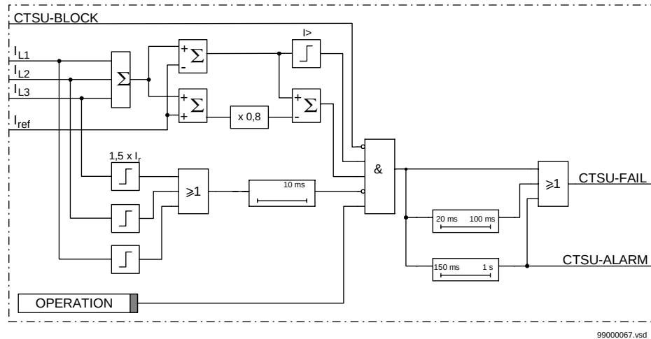
Figure 168: Simplified logic diagram for the current circuit supervision
