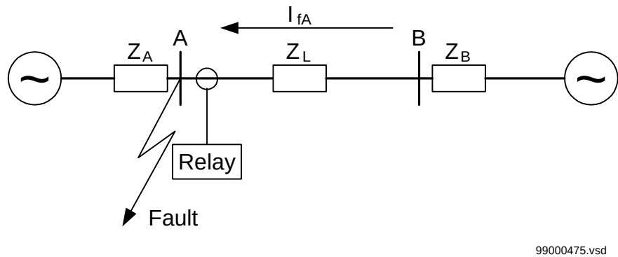
Figure 107: Through fault current from B to A: I_{fA}
