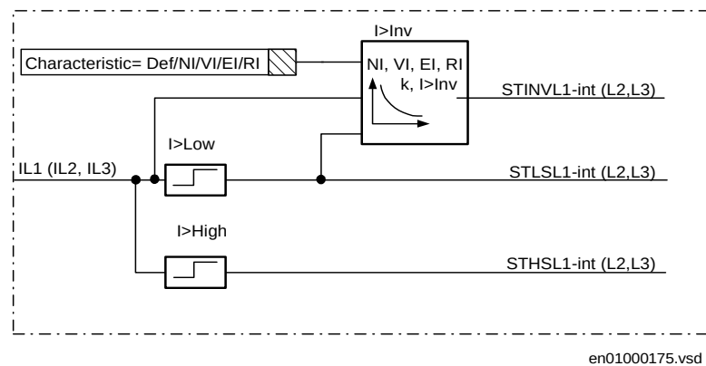
Figure 117: Simplified block diagram for definite and inverse time delayed phase overcurrent function
