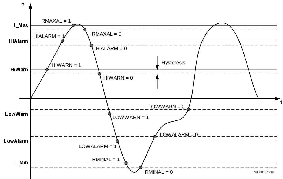
Figure 251: Presentation of the operating limits
