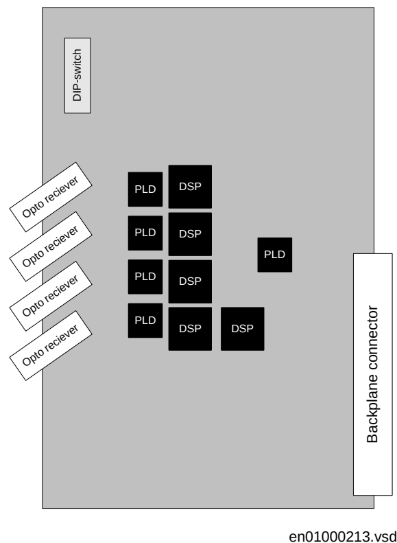
Figure 278: Block diagram for the ORM
