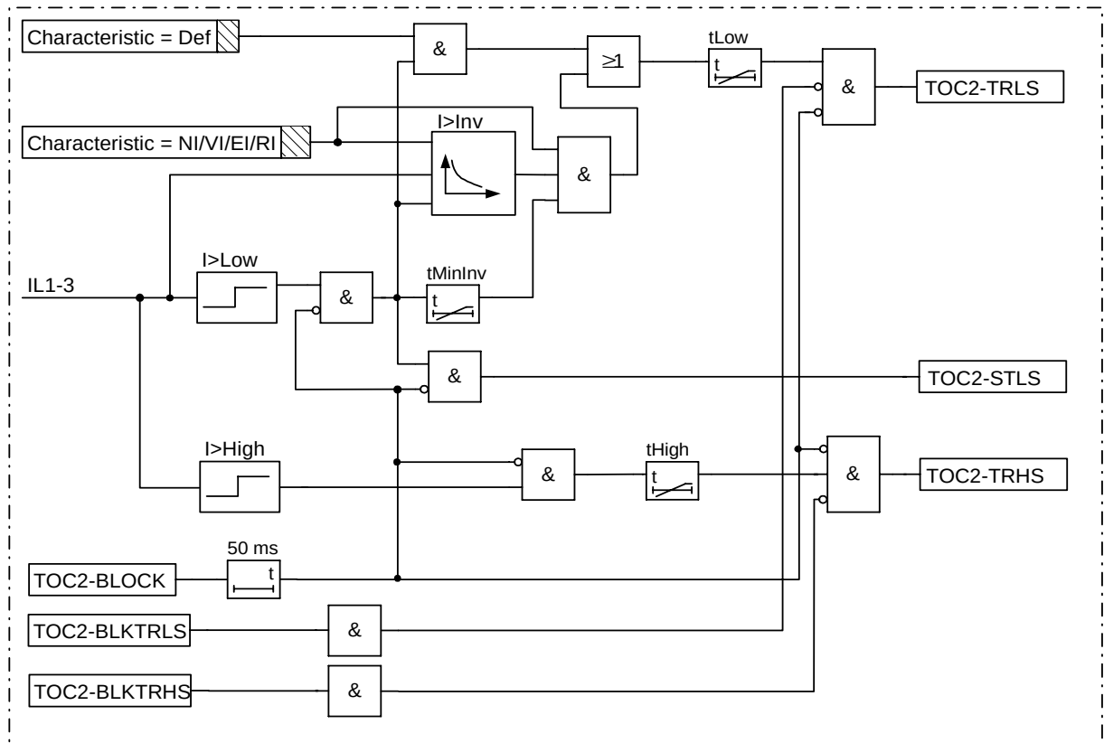
Figure 116: Two step time delayed phase overcurrent protection, simplified logic diagram
