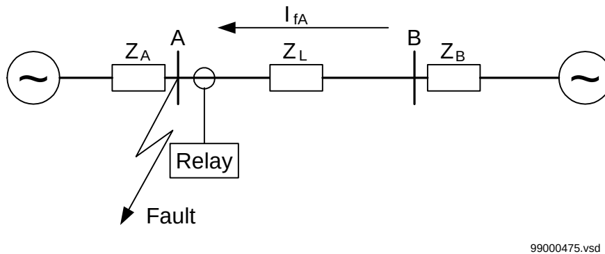
Figure 111: Through fault current from B to A: I_{fA}
