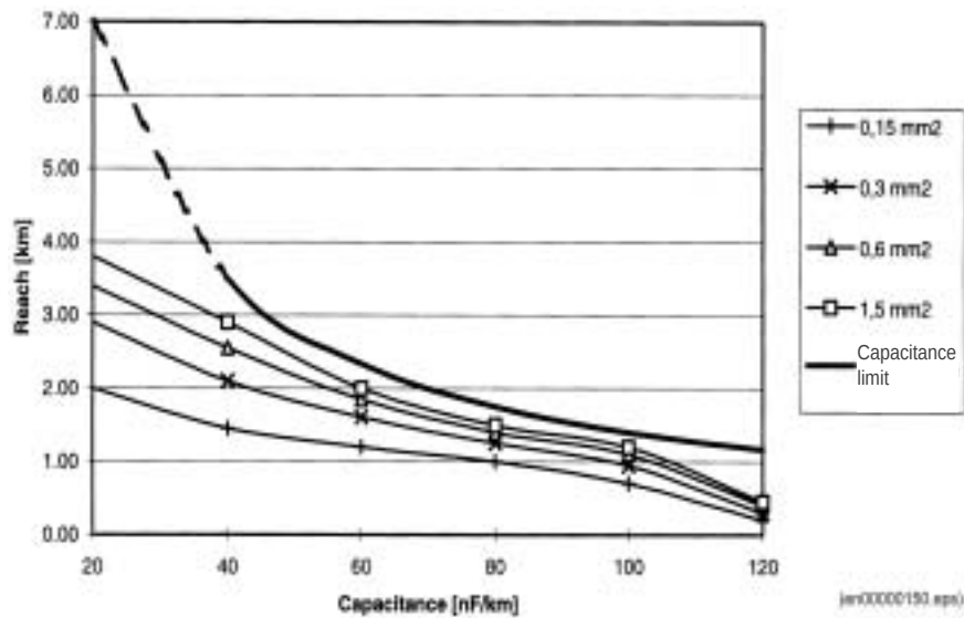
Figure 266: Maximum reach for short range galvanic modem
