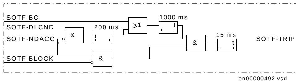
Figure 48: SOTF function - simplified logic diagram
