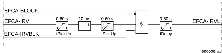
Figure 152: Simplified logic diagram, current reversal
