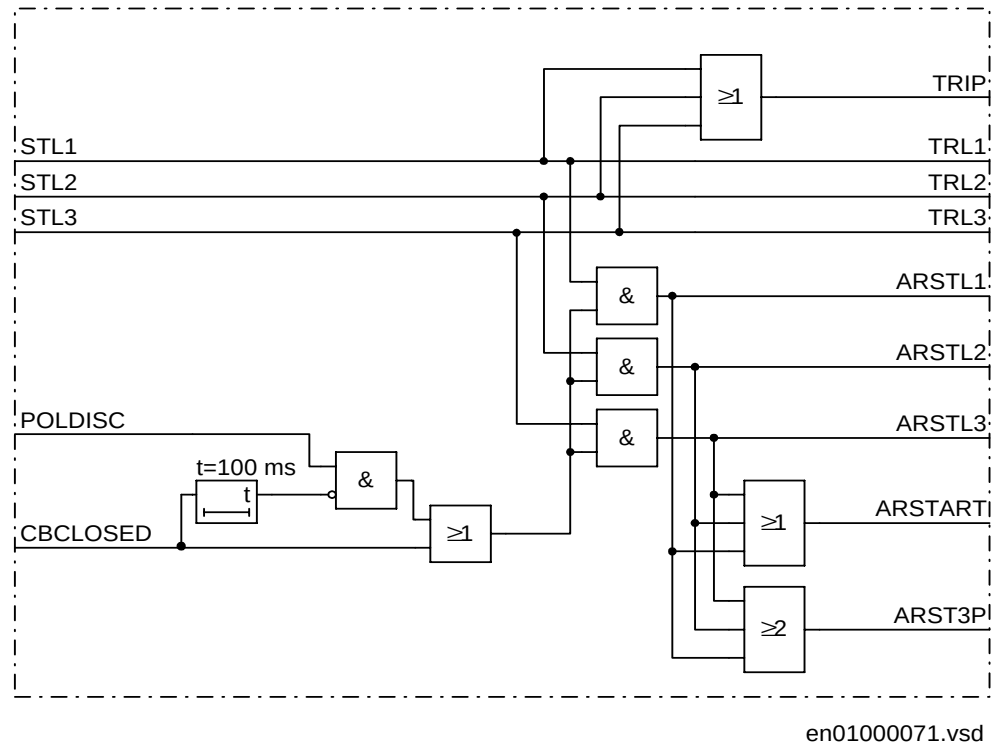
Figure 91: Trip and autorecloser start logic
