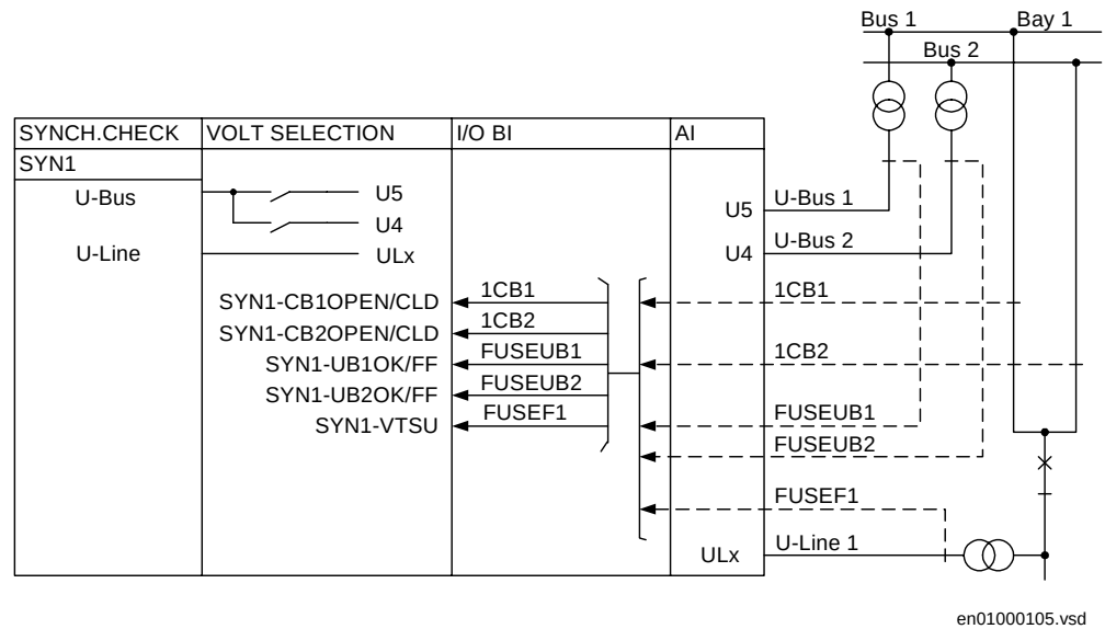
Figure 186: Voltage selection in a double bus arrangement.
