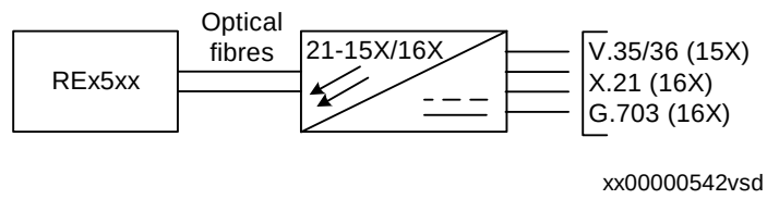
Figure 268: Multiplexed link, short range optical fibre connection
