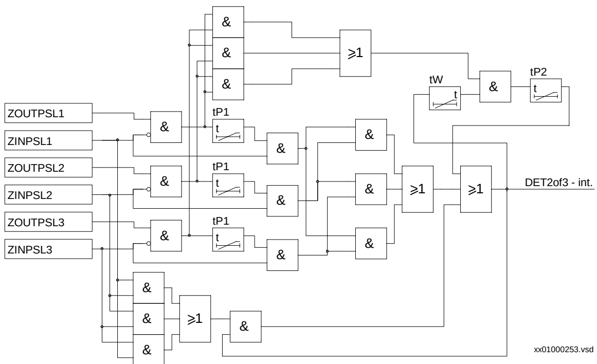
Figure 77: Simplified logic diagram for a two-out-of-three oscillation detection logic.
