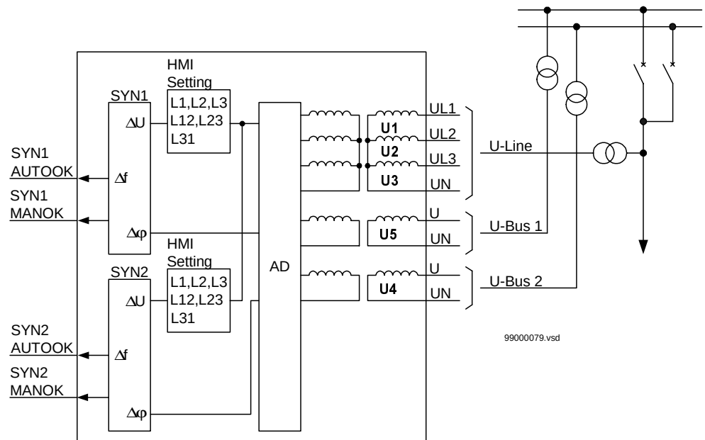
Figure 181: Connection of the synchrocheck function for one bay.
