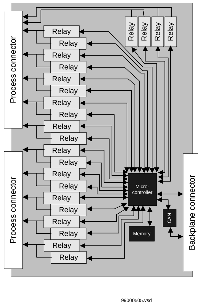
Figure 283: Block diagram of the binary output module
