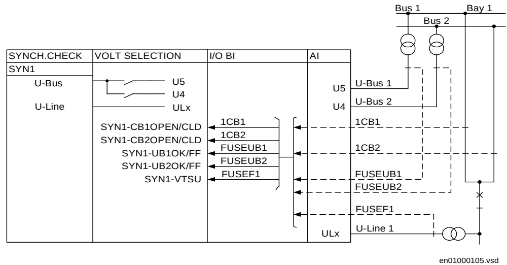
Figure 180: Voltage selection in a double bus arrangement.
