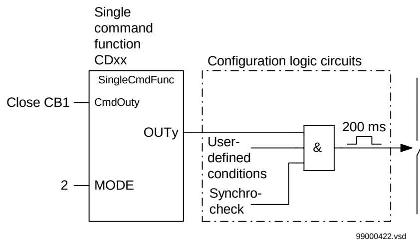
Figure 205: Application example showing a logic diagram for control of a circuit breaker via configuration logic circuits
