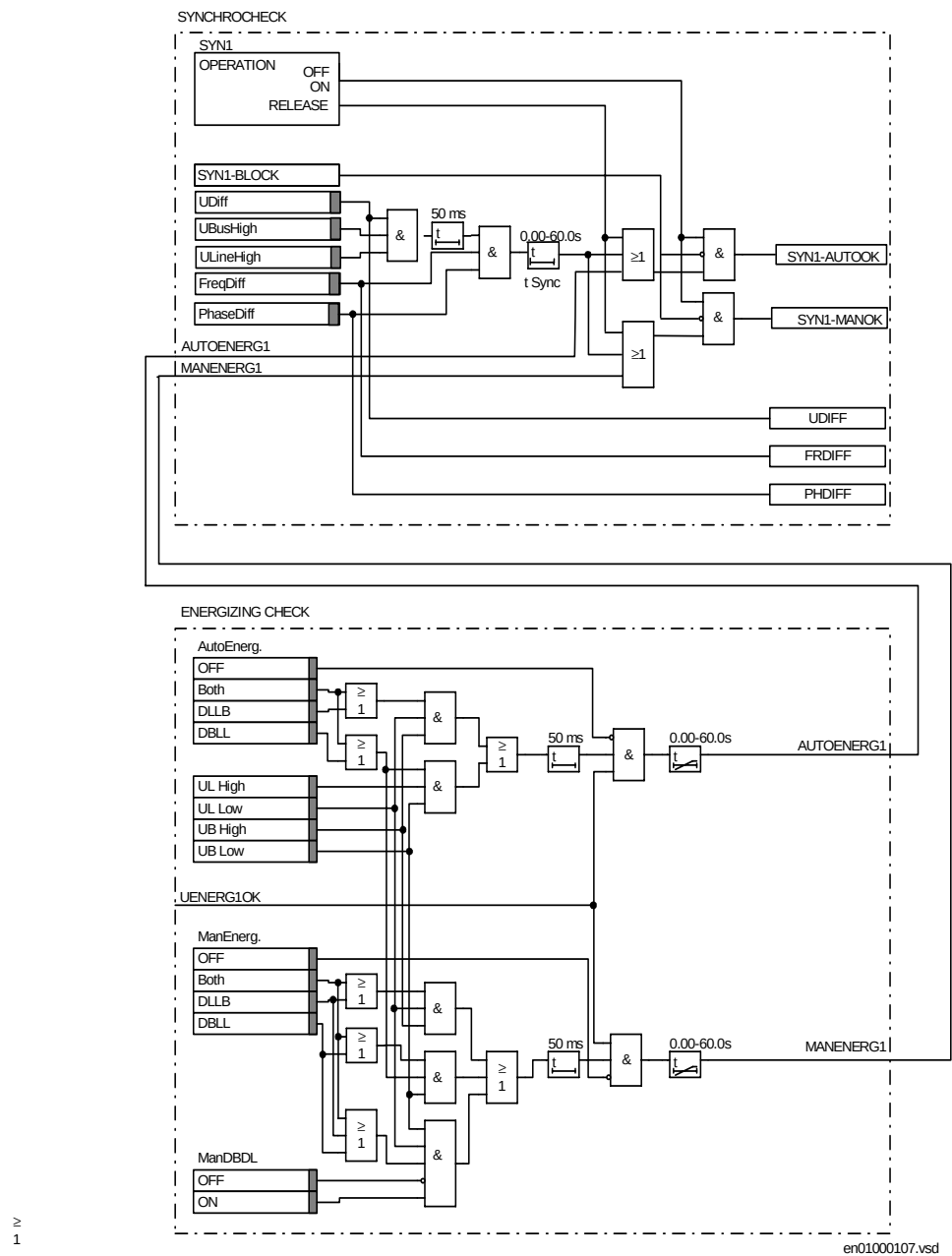
Figure 196: Simplified logic diagram - Synchrocheck and energizing check. The internal signal UENERG1OK refers to the voltage selection logic.
