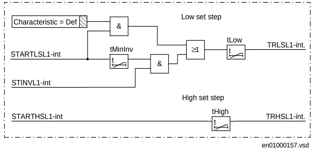
Figure 121: Delayed time operation for low set step and general time delay
