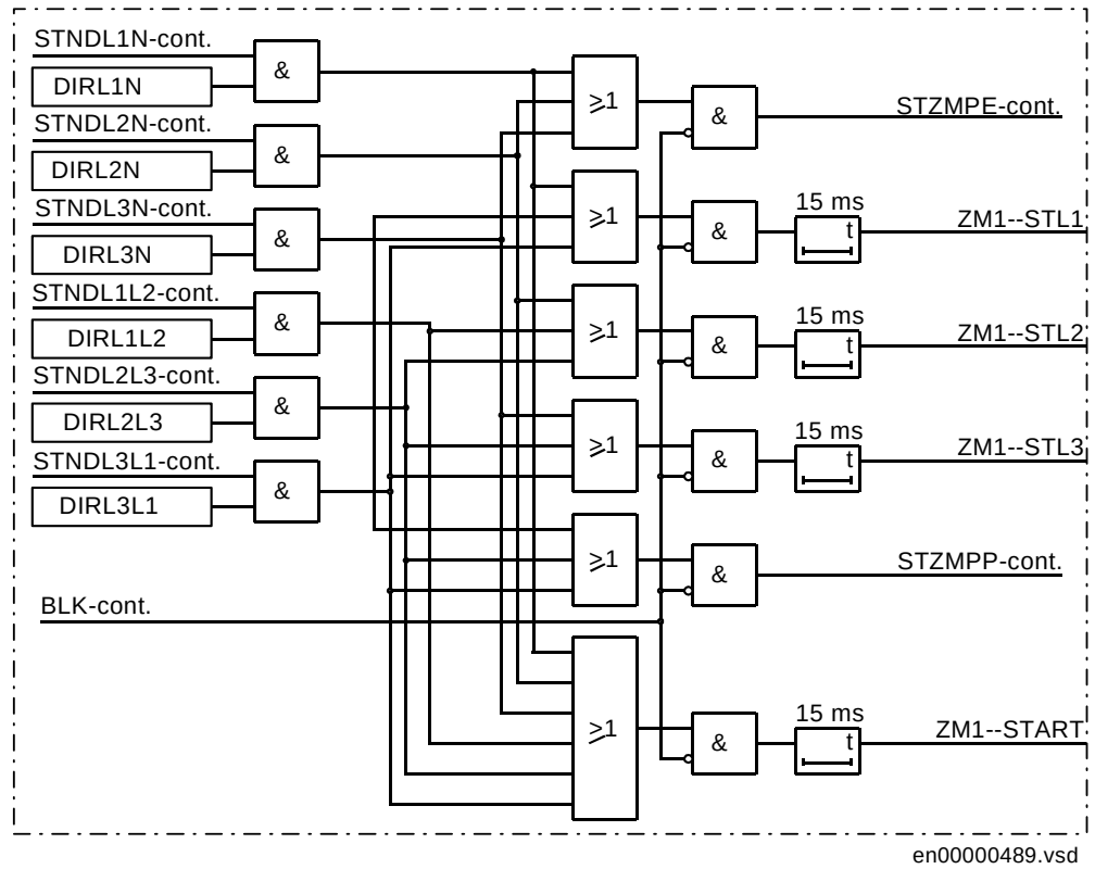
Figure 35: Composition of starting signals in directional operating mode
