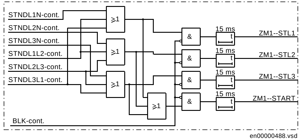
Figure 34: Composition of starting signals in non-directional operating mode
