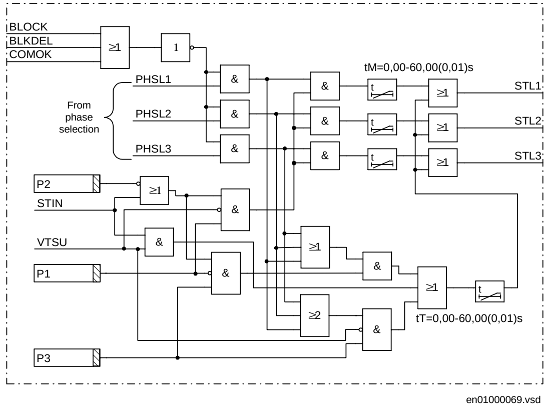
Figure 89: Function for delayed fault clearing
