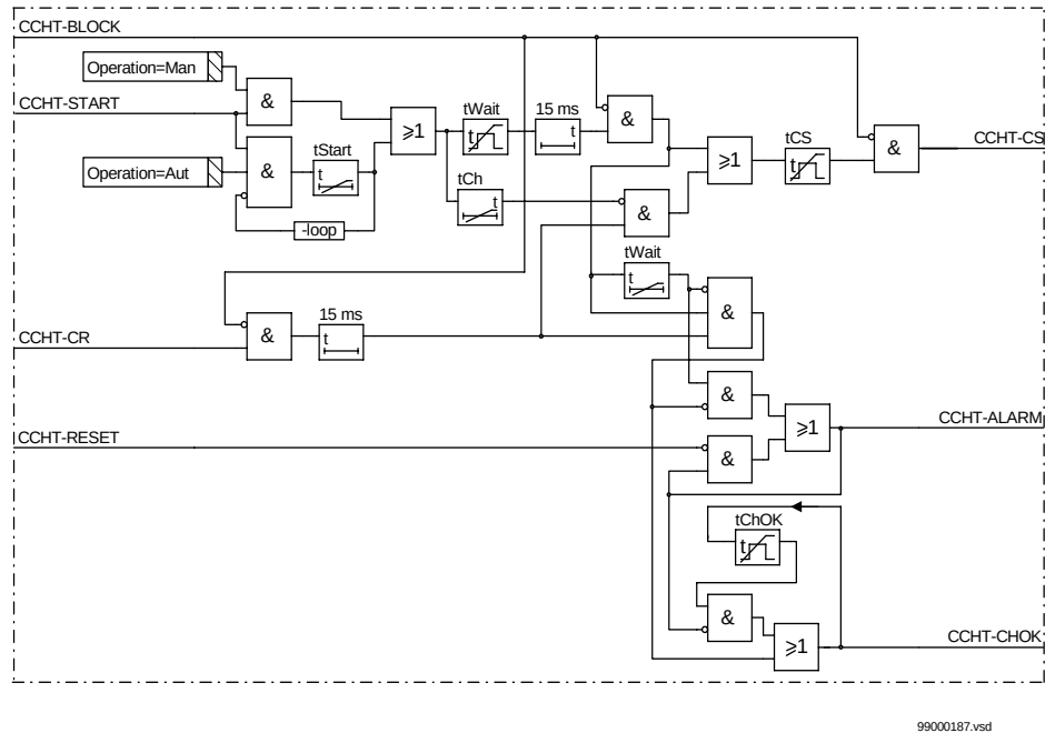
Figure 221: Simplified logic diagram for the CCHT function
