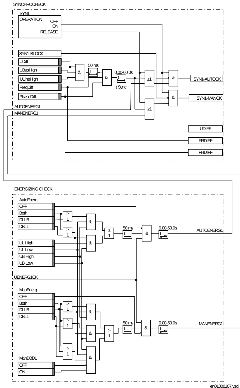
Figure 190: Simplified logic diagram - Synchrocheck and energizing check. The internal signal UENERG1OK refers to the voltage selection logic.
