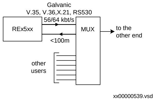
Figure 263: Multiplexed link, galvanic connection
