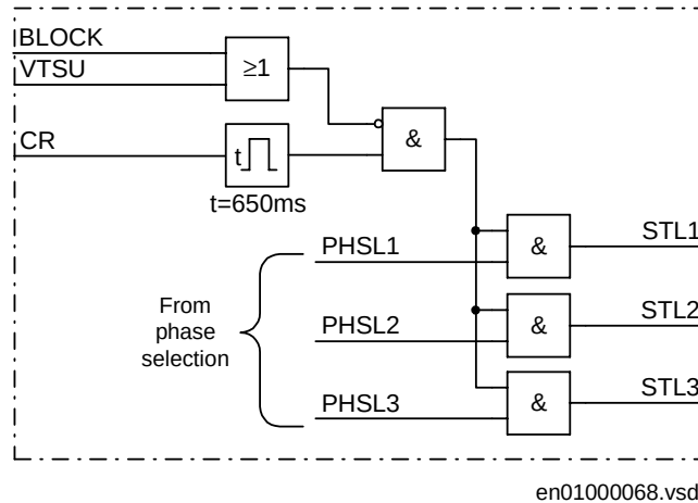
Figure 88: Function for fast fault clearing
