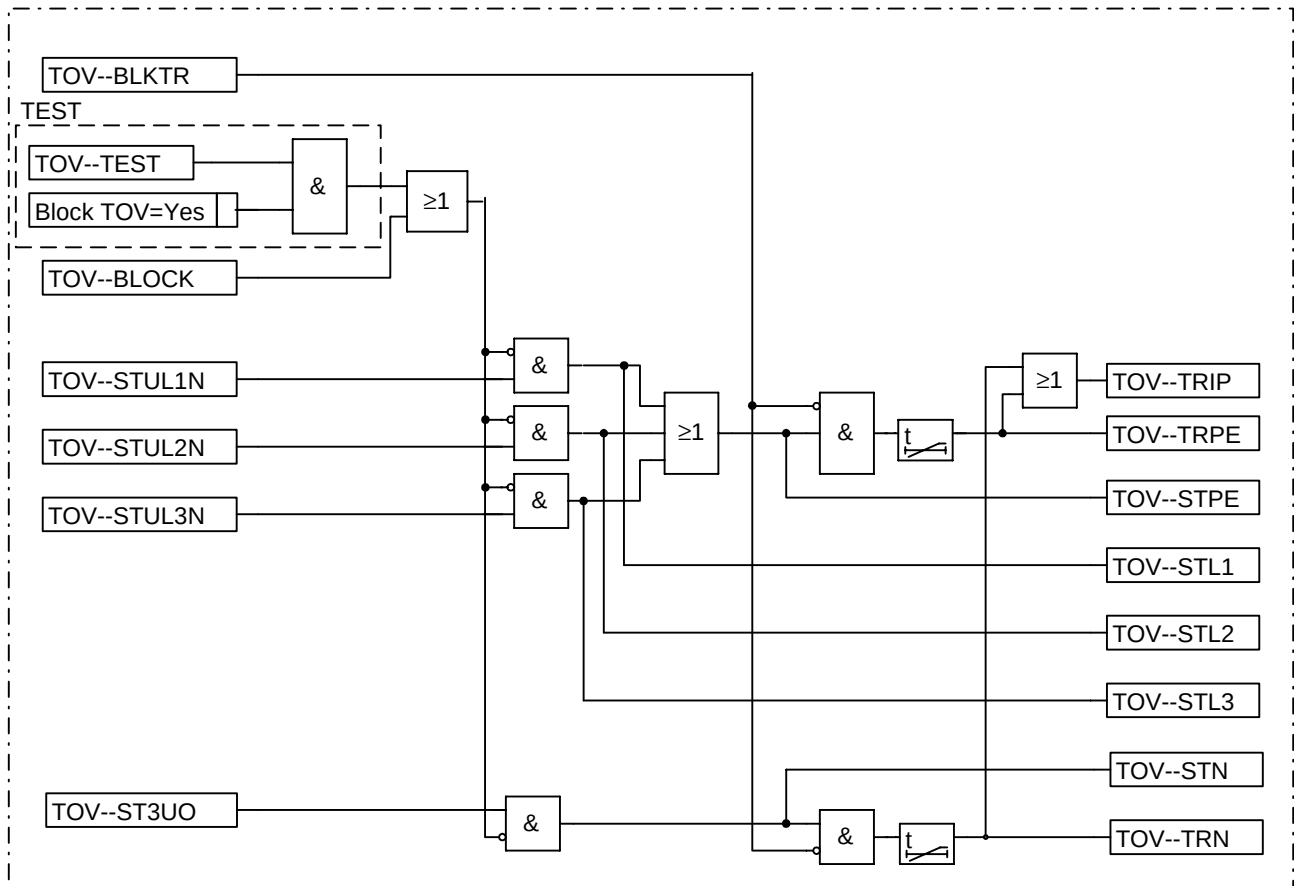
Figure 161: Time delayed overvoltage protection - simplified logic diagram
