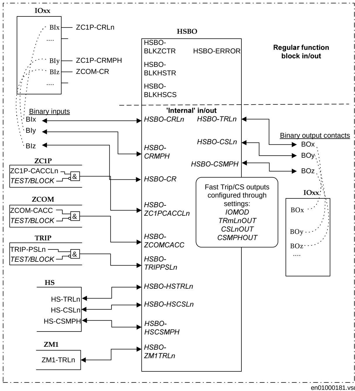
Figure 216: Simplified diagram of the high-speed binary out logic function together with depending functions
