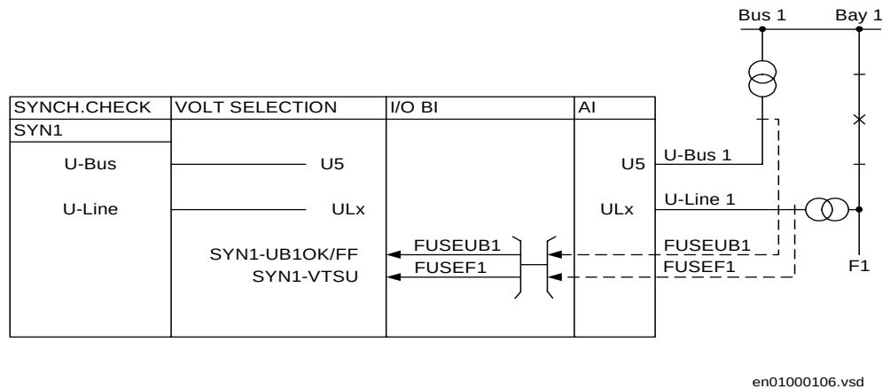
Figure 185: Voltage connection in a single busbar arrangement.
