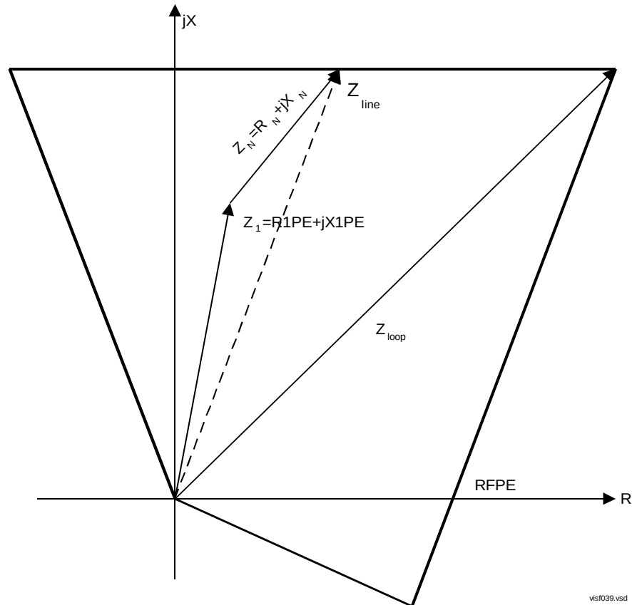
Figure 29: Characteristic of the phase-to-earth measuring loop.
