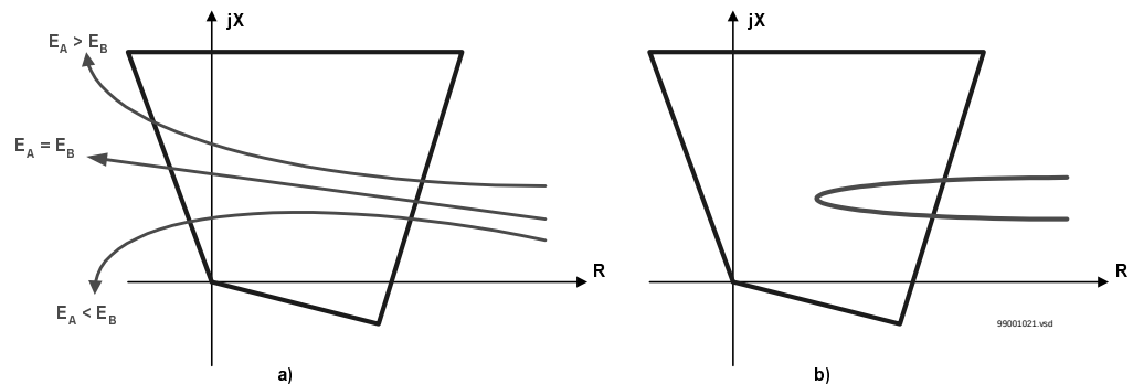
Figure 67: Impedance trajectories in relay point during the pole slip (figure a) and power swing (figure b) phenomena.
