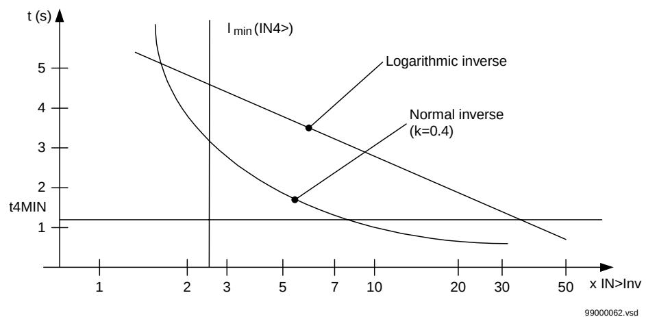
Figure 132: Normal inverse and logarithmic inverse time characteristics.
