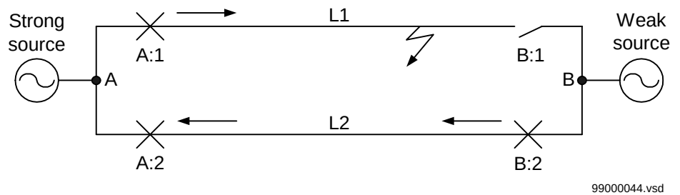
Figure 100: Current distribution after the breaker B:1 is opened.
