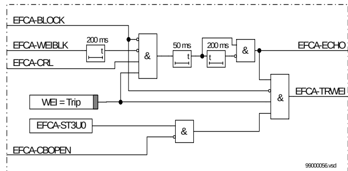
Figure 151: Simplified logic diagram, weak end infeed - Trip.
