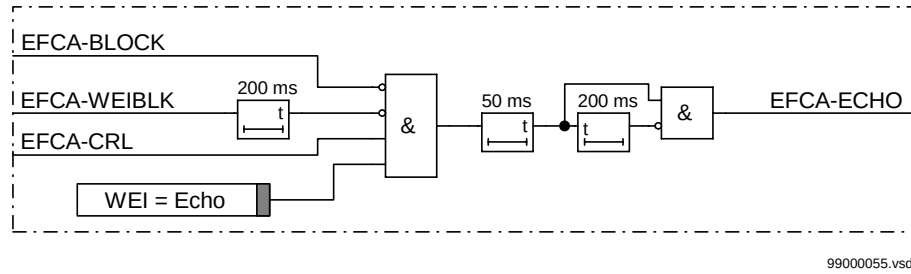
Figure 150: Simplified logic diagram, weak end infeed - echo.
