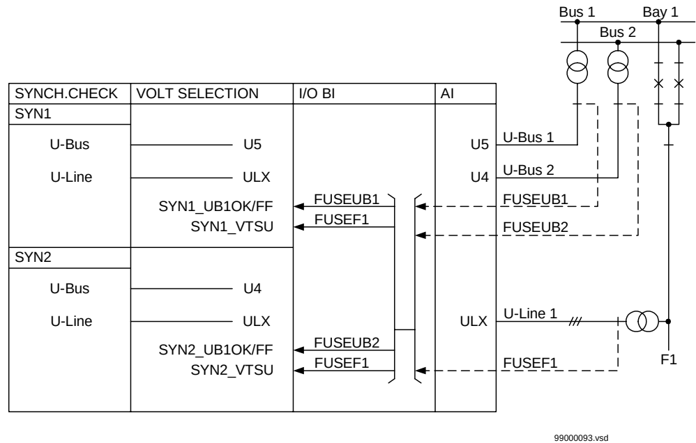
Figure 188: Voltage connection in a double breaker arrangement.
