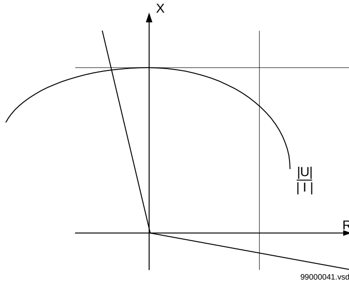
Figure 47: Basic operating characteristic
