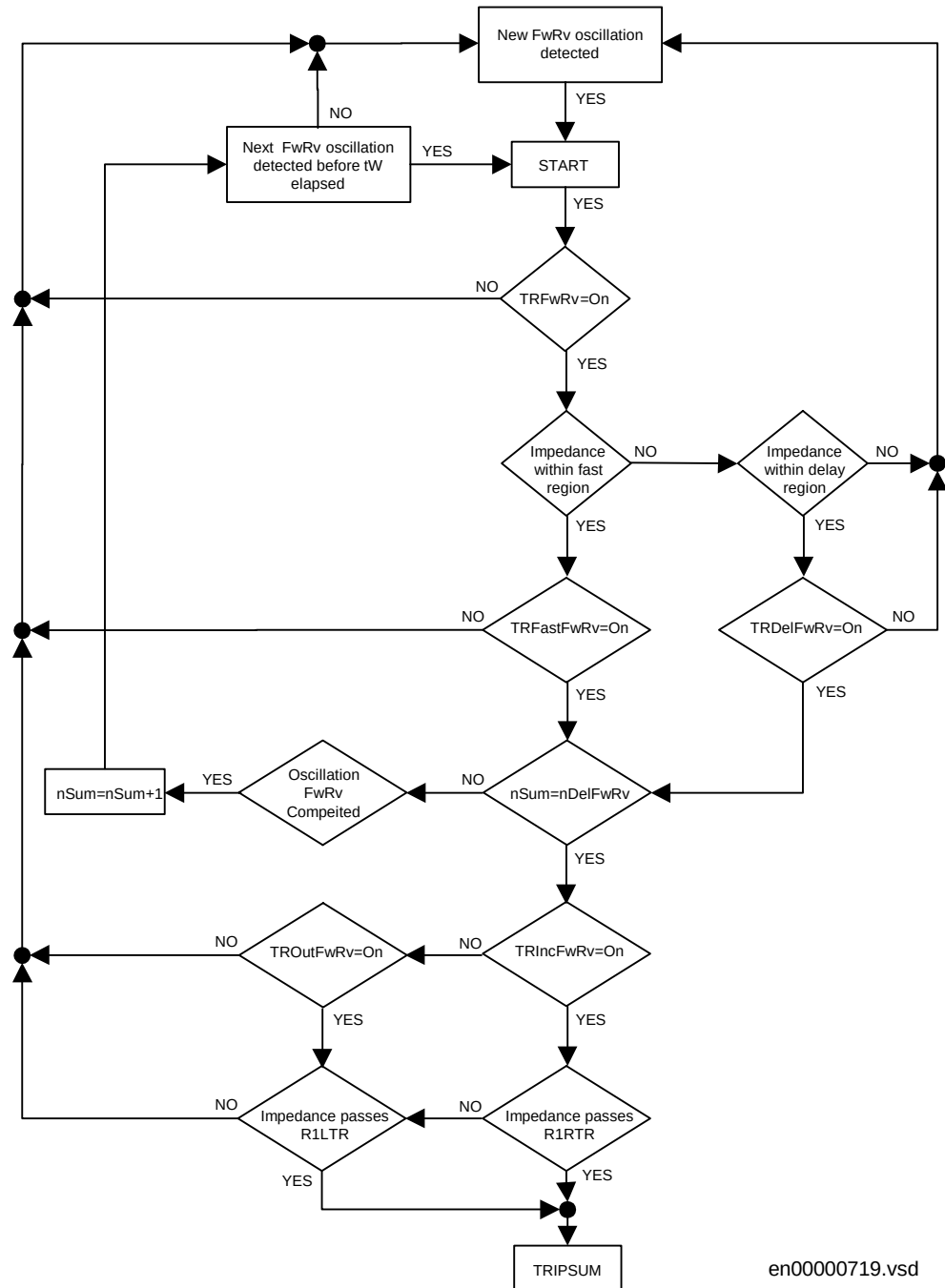
Figure 82: Flow-chart presenting summation trip (TRIPSUM) of the pole slip protection for the forward to reverse transition (FwRv).
