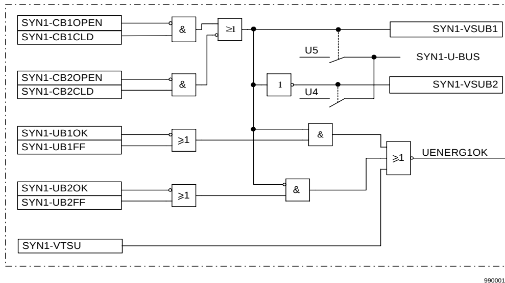
Figure 191: Voltage selection logic in a double bus, single breaker arrangement. In case of three bay arrangement the 1 in SYN1 and UENERG1OK are replaced by 2 and 3 in the logic.
