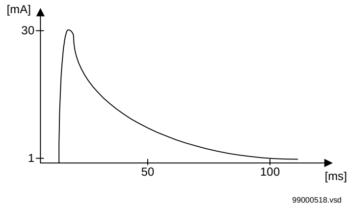
Figure 281: Current through the relay contact
