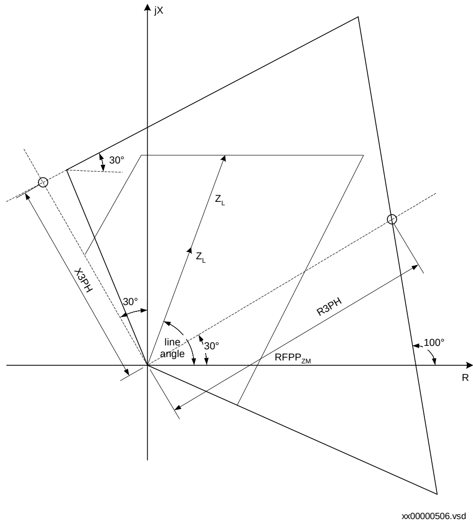
Figure 55: Phase selection operate characteristic at three-phase faults.
