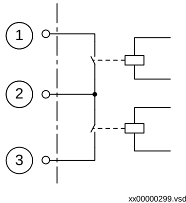
Figure 284: One of twelve binary output groups
