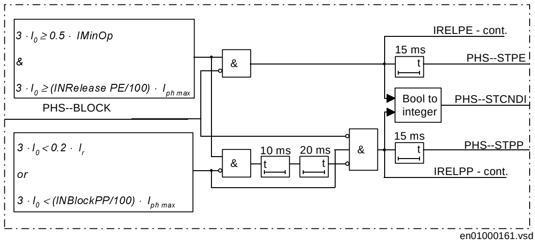
Figure 49: Ph-Ph and Ph-E operating conditions.
