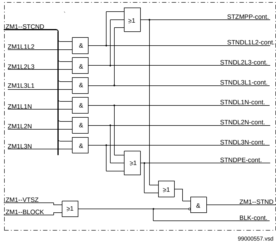
Figure 33: Conditioning by a group functional input signal ZM1--STCND
