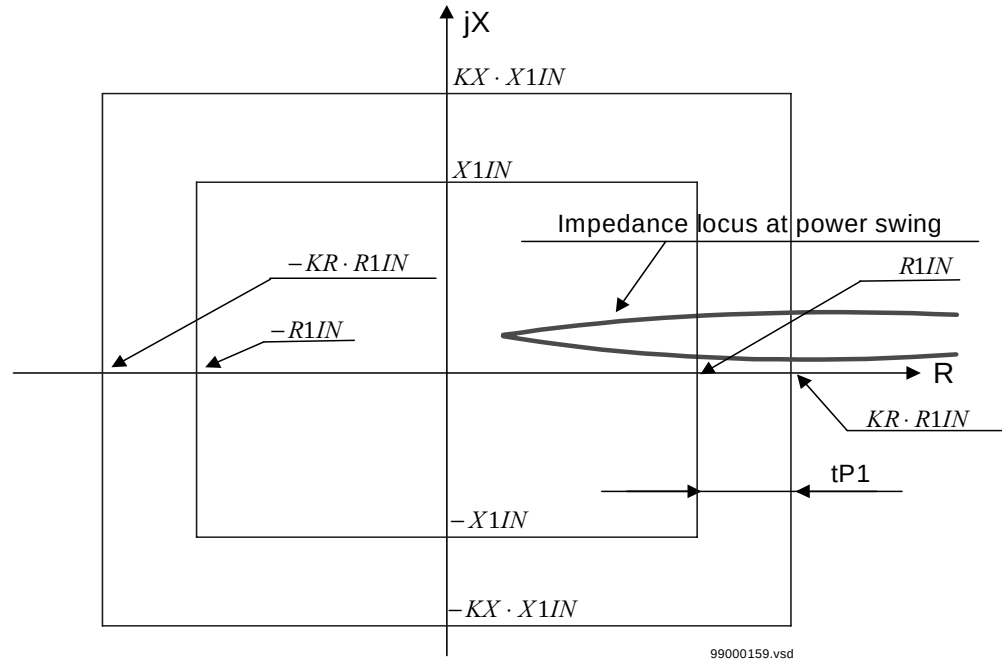
Figure 57: Operating principle and characteristic of the PSD function.
