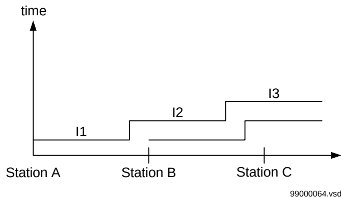
Figure 138: Example of selectivity plan for the directional current steps.
