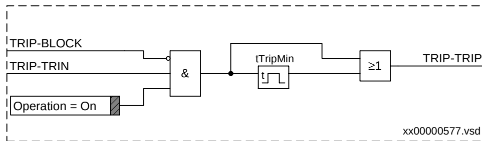
Figure 208: Simplified logic diagram for trip logic
