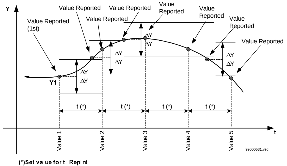
Figure 247: Periodic reporting with amplitude dead-band supervision in parallel.
