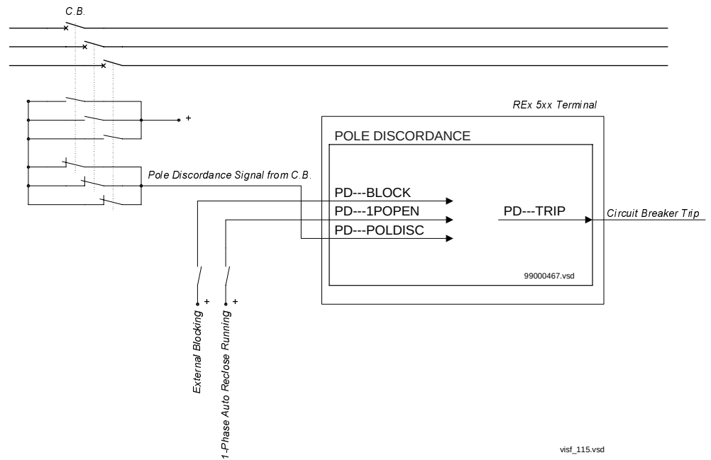
Figure 214: Typical connection diagram for pole discordance function - contact based
