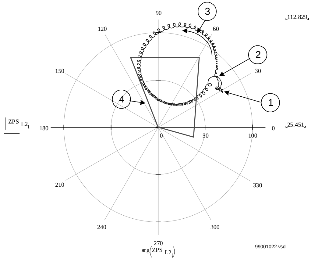
Figure 68: Impedance trajectory as seen by a L2-N impedance measuring element.
