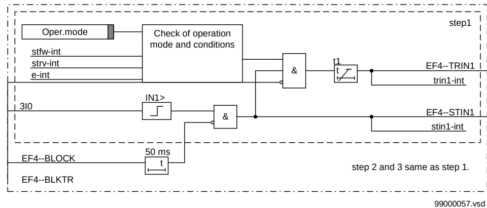
Figure 127: Simplified logic diagram of internal function Step 1. Step 2 and step 3 are the same.
