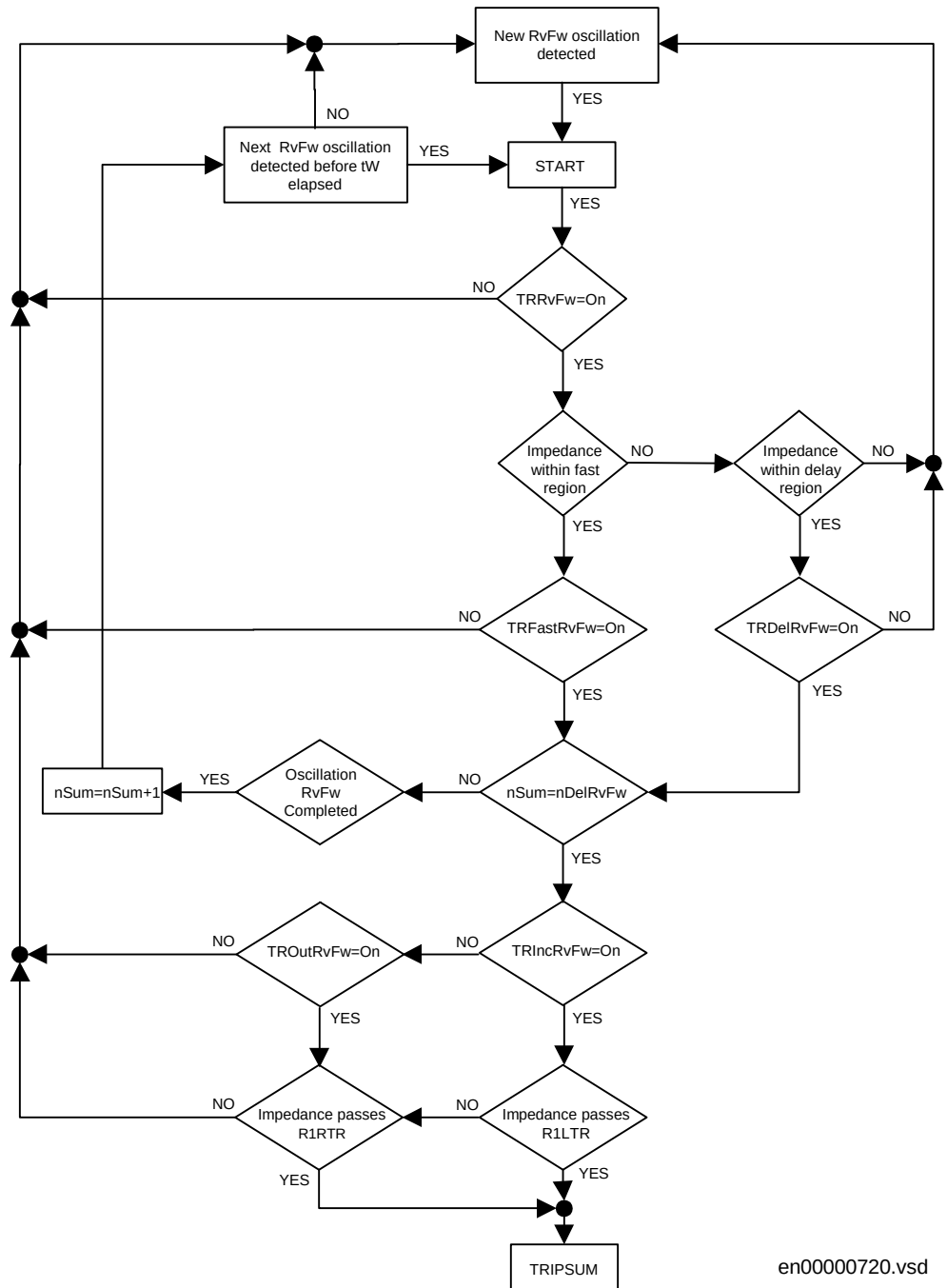
Figure 83: Flow-chart presenting summation trip (TRIPSUM) of the pole slip protection for the reverse to forward transition (RvFw).
