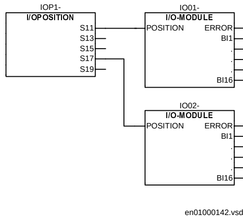
Figure 3: Example of an I/O-configuration in the graphical CAP tool for a REx 5xx with two BIMs.
