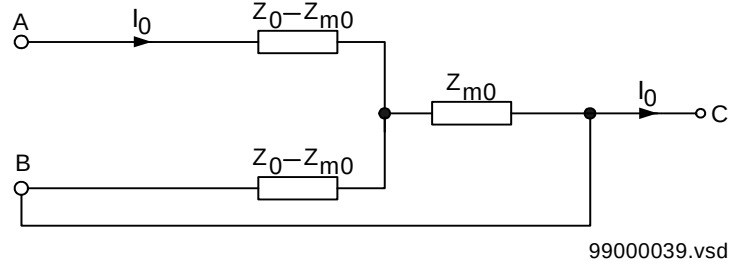
Figure 41: Equivalent zero-sequence impedance circuit for the double-circuit line that operates with one circuit disconnected and earthed at both ends
