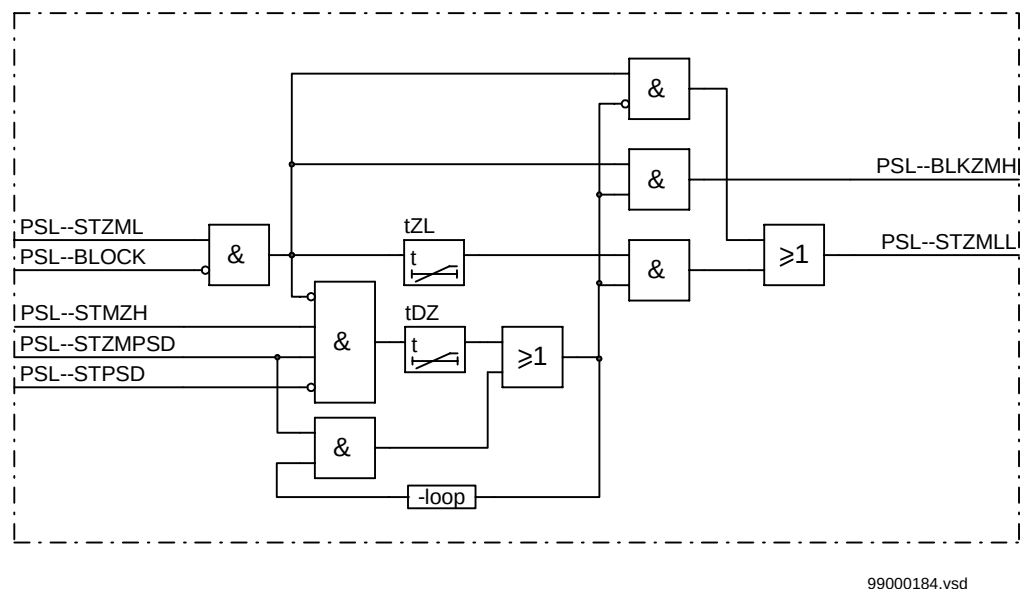
Figure 64: Control of the underreaching distance protection zone (zone 1) at power swings caused by the faults on remote lines.
