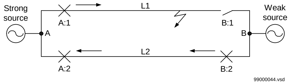
Figure 147: Current distribution after the breaker at B:1 is opened
