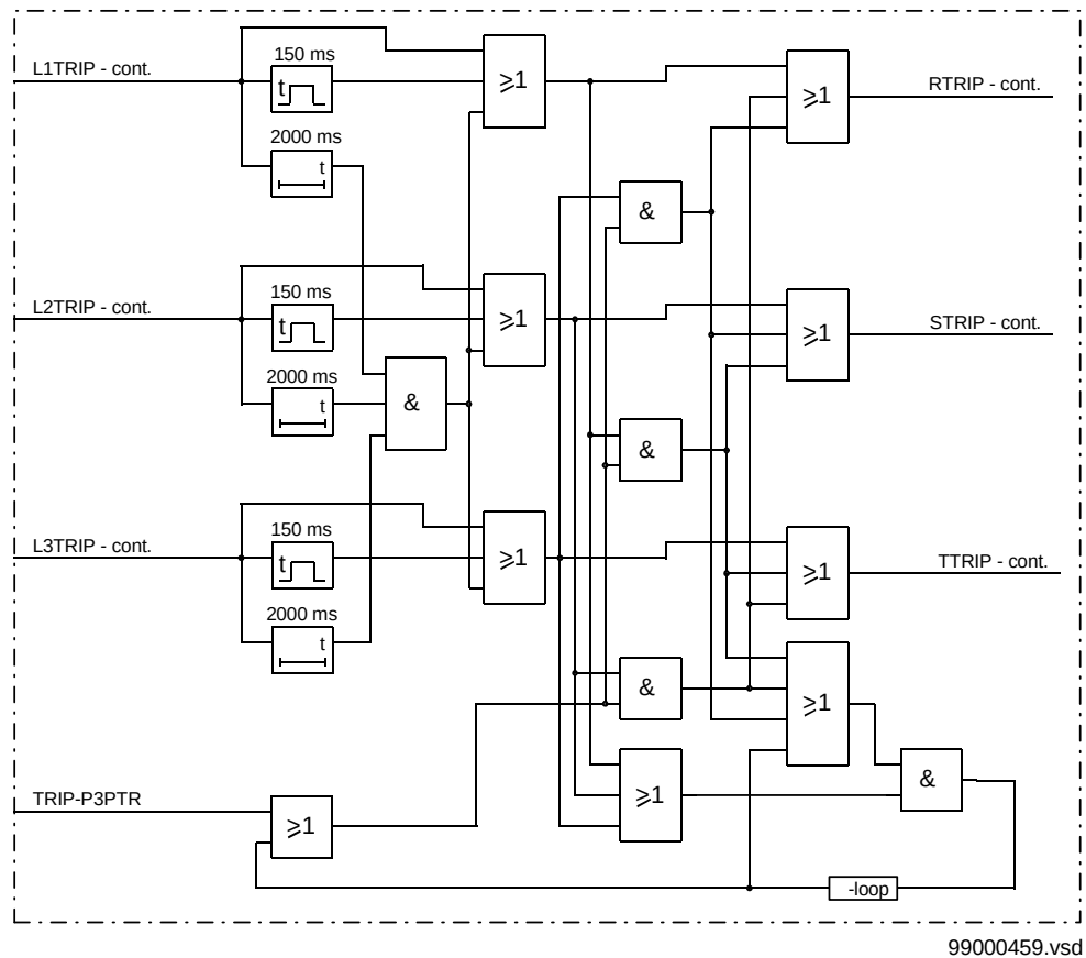
Figure 212: Additional logic for the 1ph/2ph/3ph operating mode
