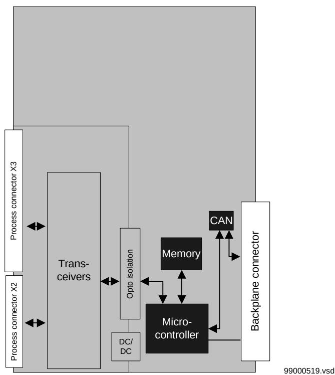
Figure 264: Block diagram for the galvanic communication module
