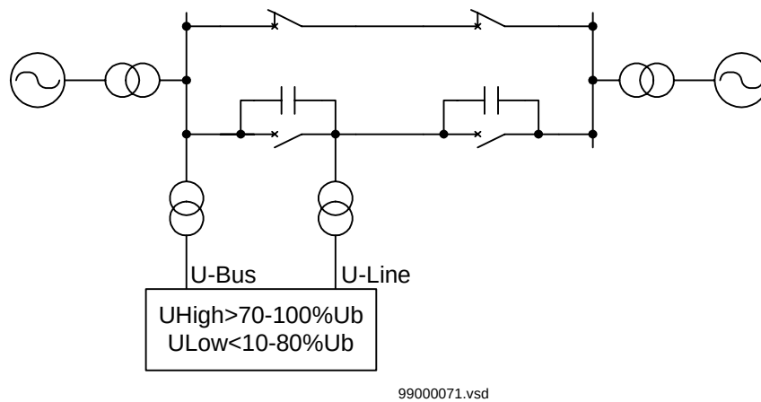
Figure 178: Principle for energizing check.
