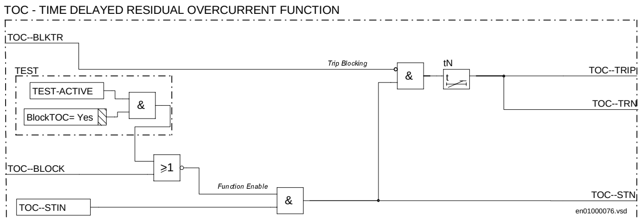
Figure 115: Simplified logic diagram of the TOC-- protection function.
