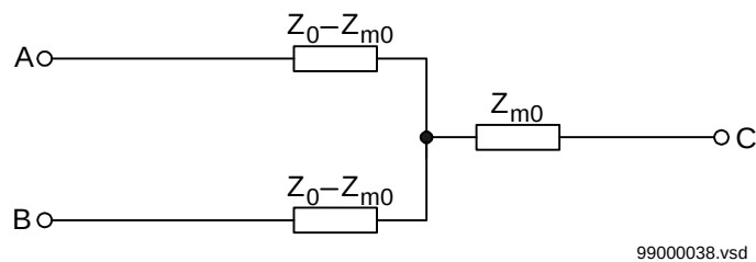
Figure 40: Equivalent zero sequence impedance circuit of the double-circuit, parallel, operating line with a single phase-to-earth fault at the remote busbar
