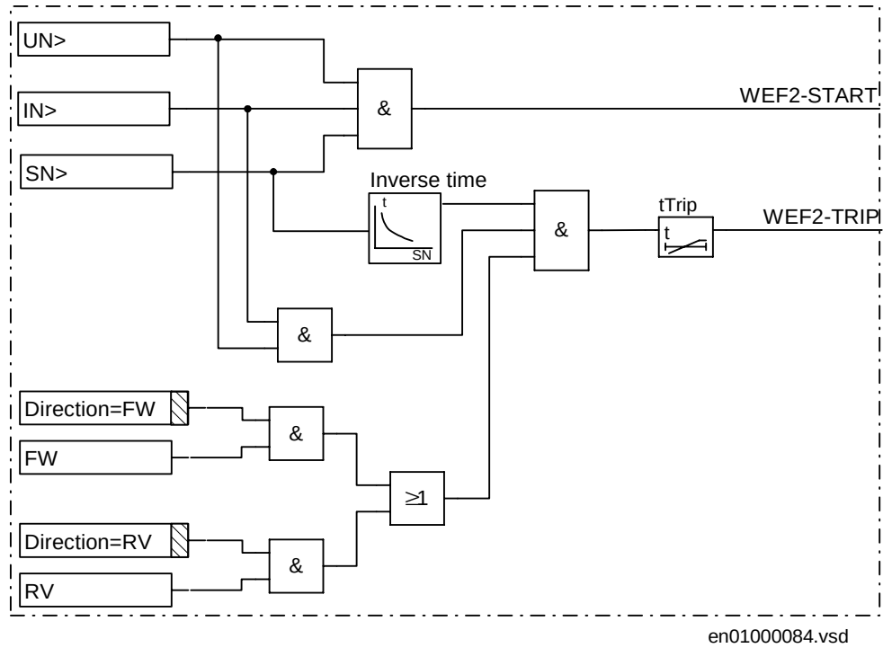
Figure 142: Logic for sensitive directional residual power protection function (WEF2)
