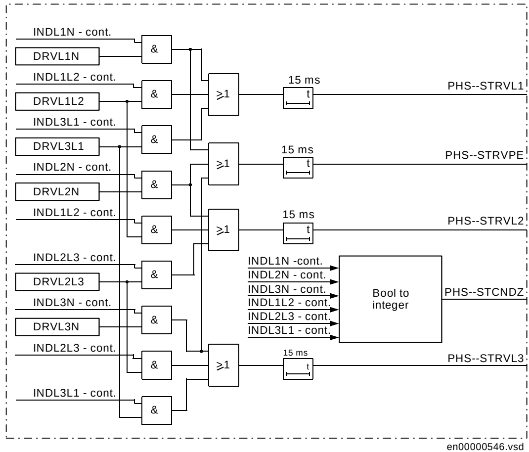
Figure 51: Composition of non directional phase selection signals
