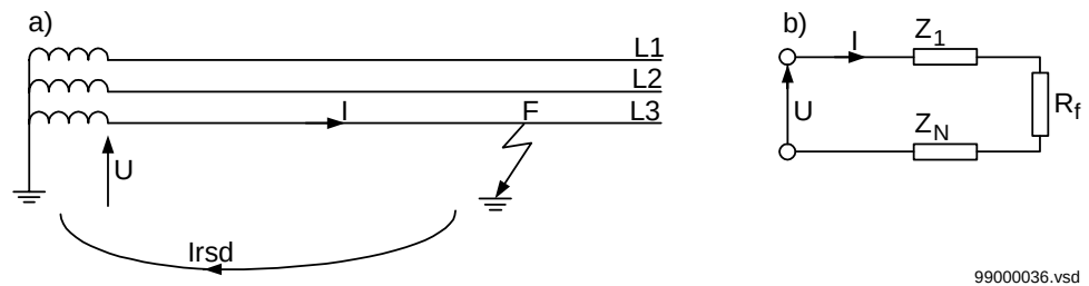
Figure 38: Equivalent circuits for measurement at single-phase-to-earth faults.
