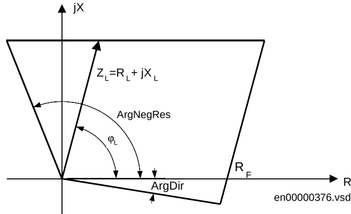
Figure 27: Typical characteristic of a distance protection zone.
