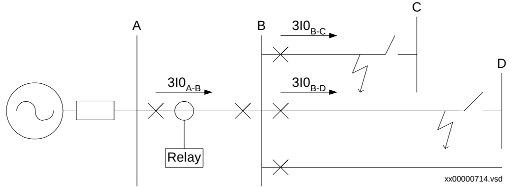
Figure 137: Example of fault cases between stations. Calculation of 3I0_{min} for step 2 (and step 3).
