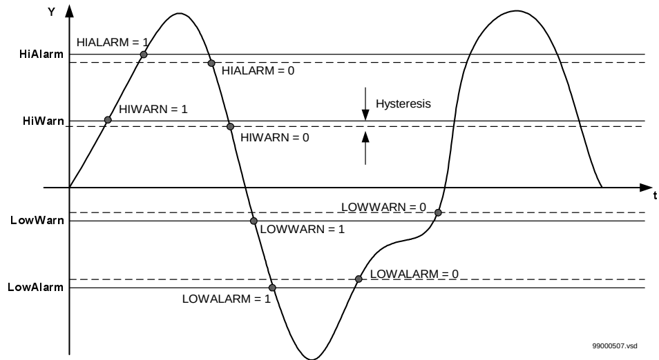
Figure 243: Presentation of the operating limits.
