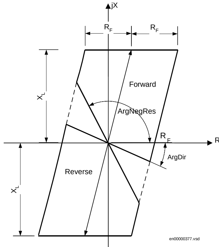
Figure 28: Nondirectional and directional (forward and reverse) operating characteristic
