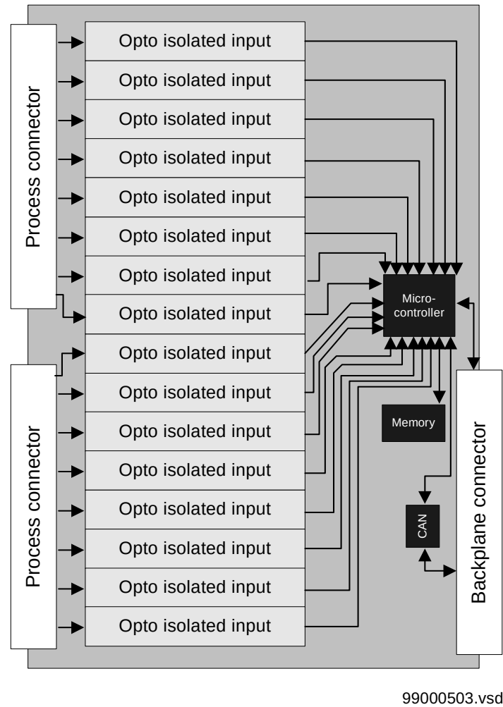
Figure 282: Block diagram of the binary input module
