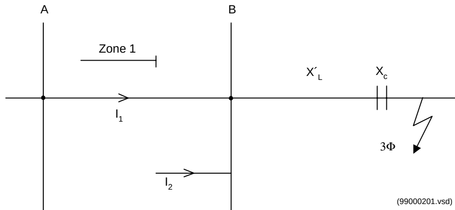
Figure 45: Series compensated and adjacent line
