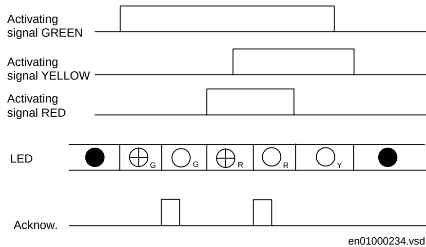
Figure 230: Operating sequence 3, three colors involved, alternative 2
