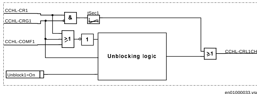
Figure 218: Communication channel logic 1
