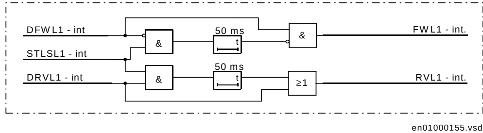
Figure 119: Current reversal logic for one phase and one set step
