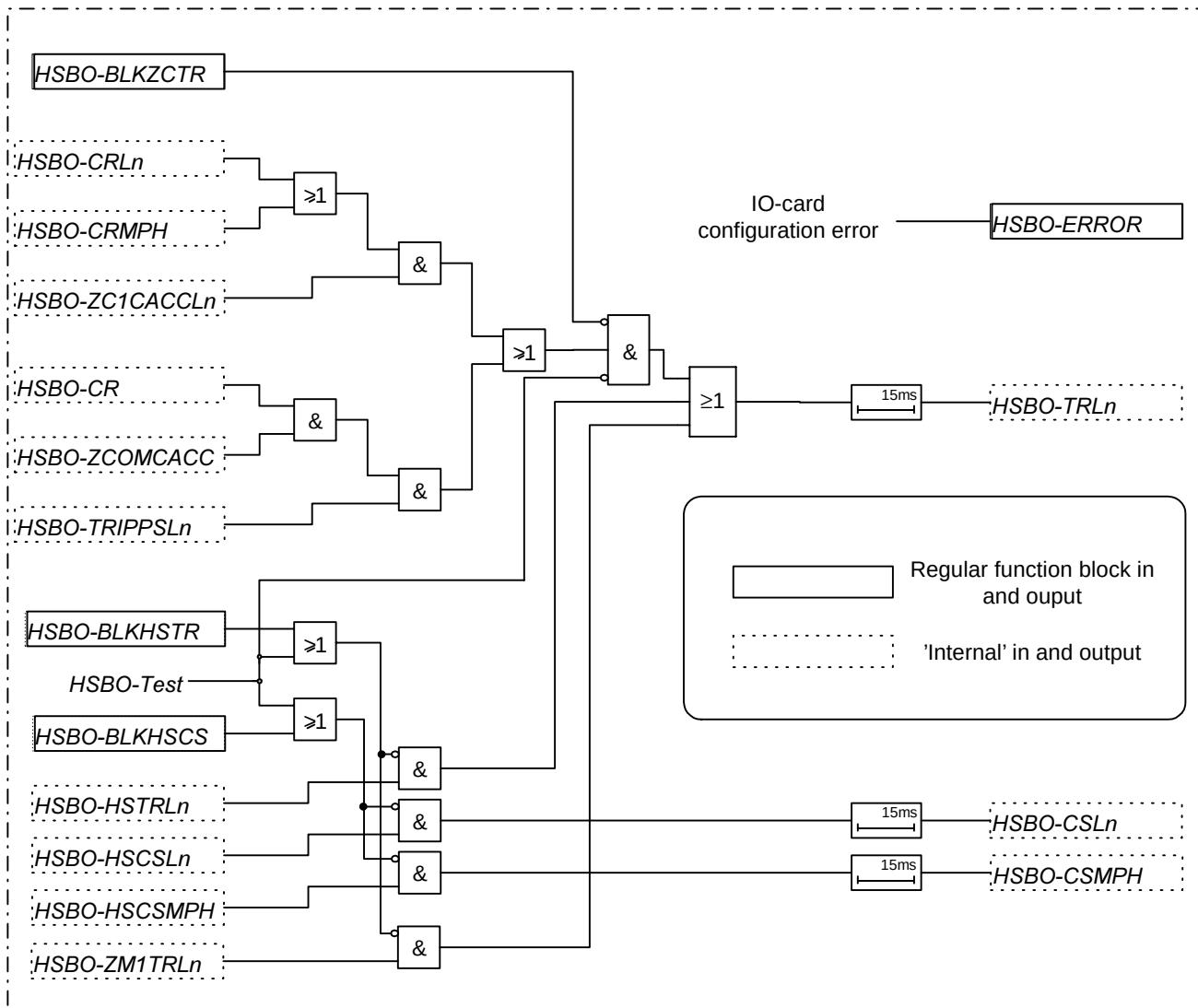
Figure 217: Simplified logic diagram of the function block
