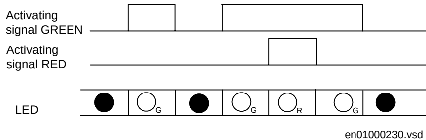
Figure 226: Operating sequence 1, two colors
