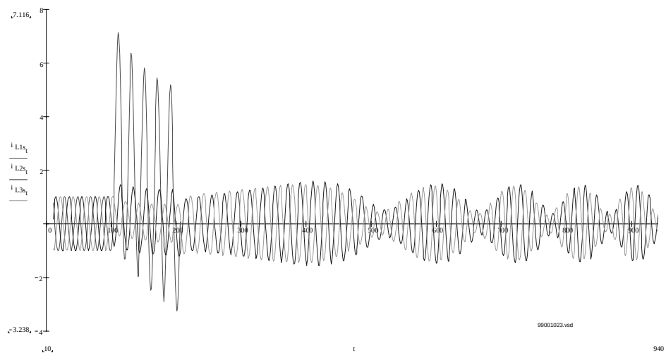
Figure 69: Phase currents in relay point during the pole slip conditions caused by a L1-N fault.
