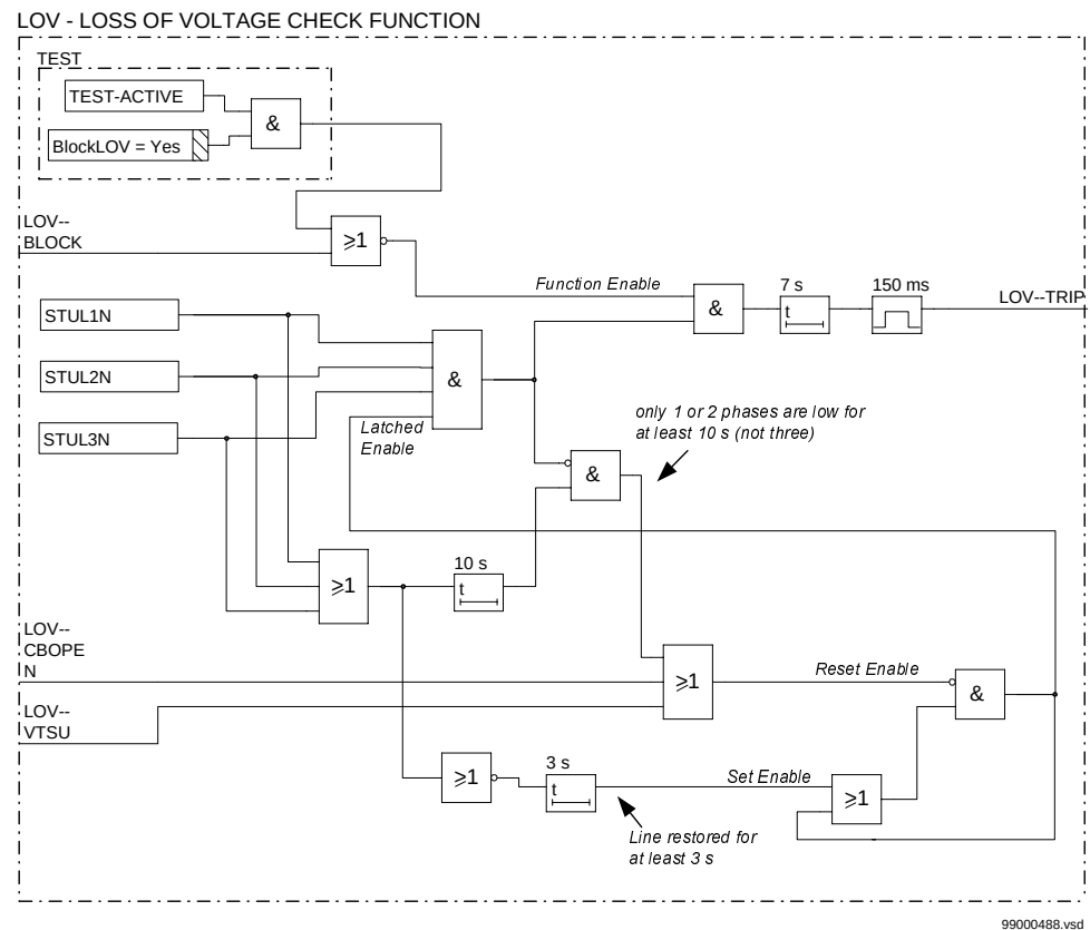
Figure 165: Simplified logic diagram of loss of voltage check protection function
