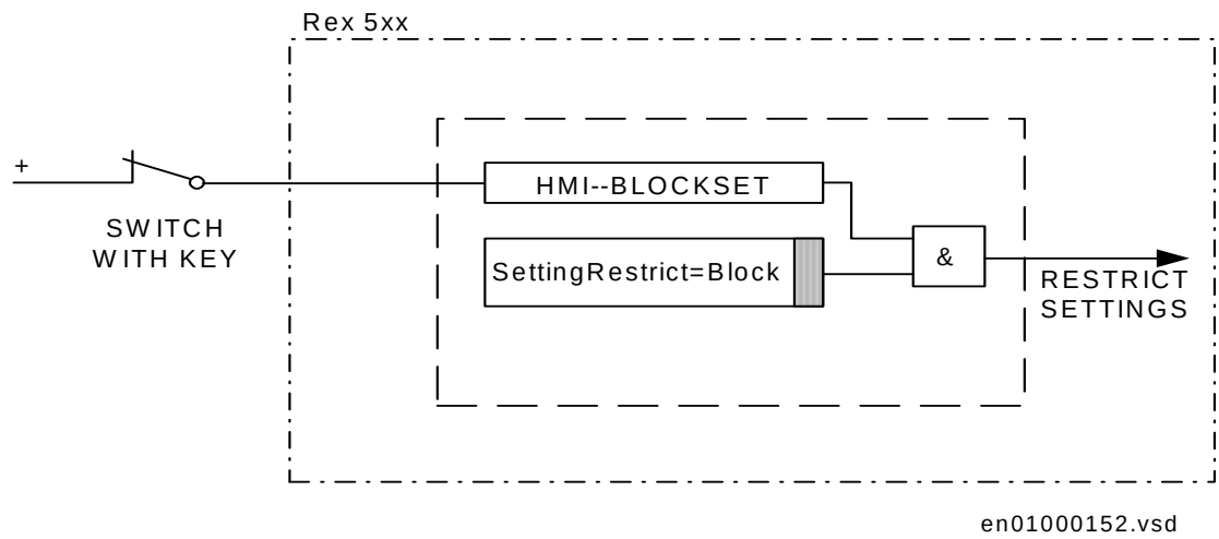
Figure 1: Connection and logic diagram for the BLOCKSET function
