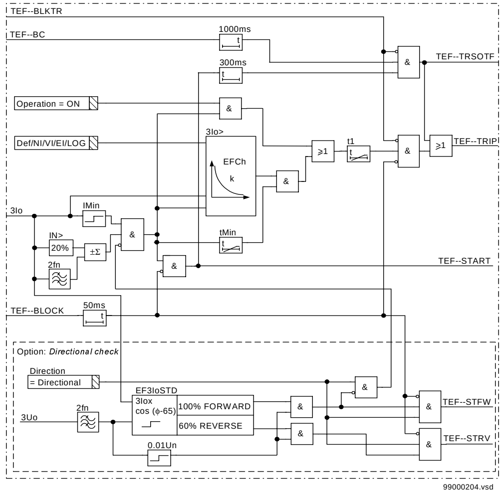
Figure 124: Simplified logic diagram for the residual overcurrent protection
