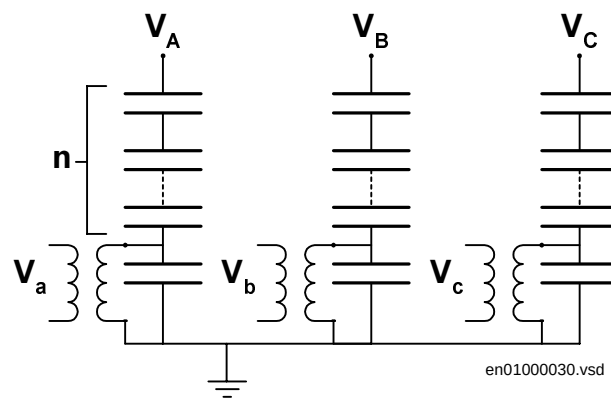
Figure 174: Capacitive voltage transformer
