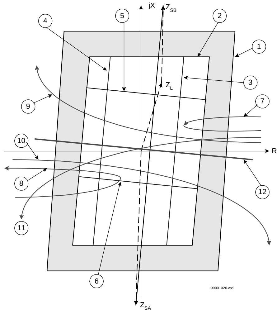
Figure 72: Impedance trajectories during oscillations in power system and basic operating characteristics of the pole slip protection.
