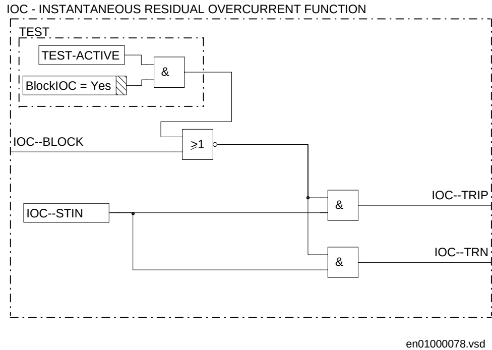
Figure 105: Simplified logic diagram of instantaneous residual overcurrent protection.
