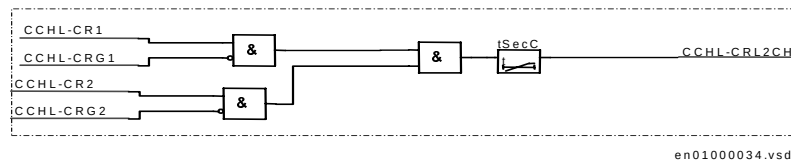
Figure 219: Combination of two communication channels
