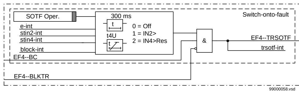
Figure 128: Simlified logic diagarm of internal function Switch-onto-fault.
