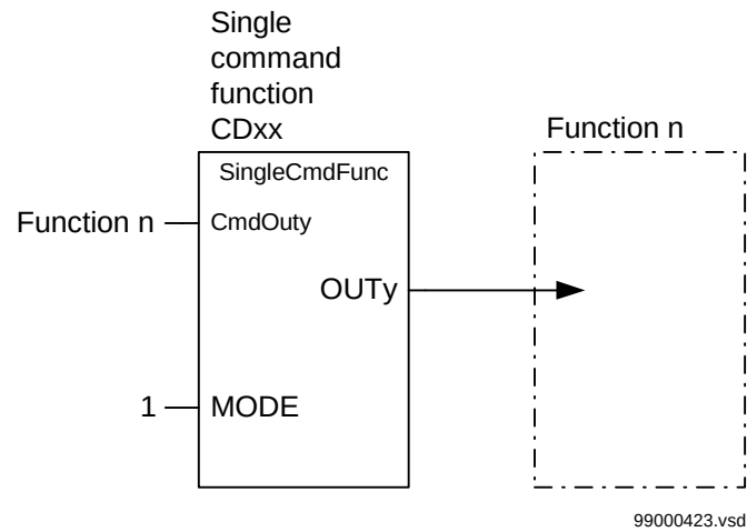
Figure 206: Application example showing a logic diagram for control of built-in functions
