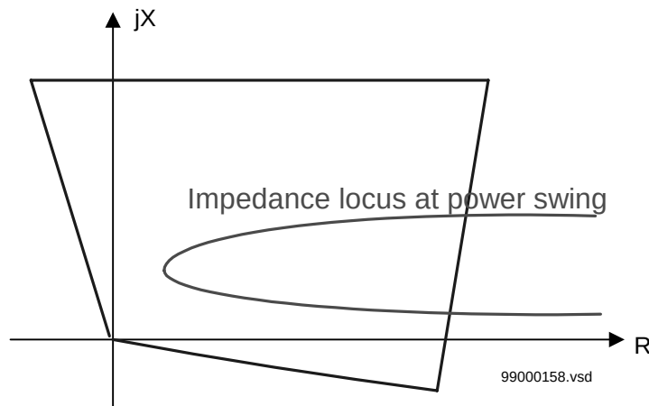
Figure 56: Impedance plane with the locus of the measured impedance and operate characteristics of the zone measuring elements.
