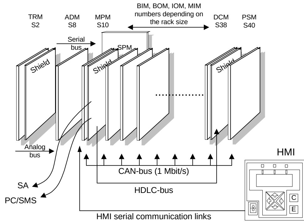
Figure 272: Internal hardware structure showing a full width case configuration
