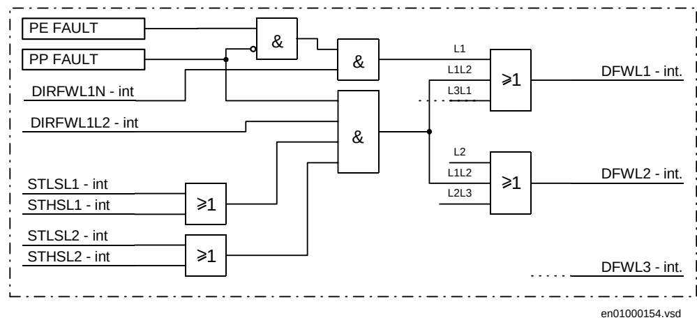
Figure 118: Excerpt from directional phase selection
