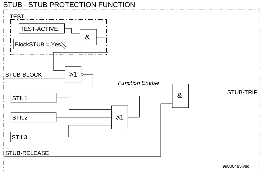
Figure 154: Simplified logic diagram of stub protection.
