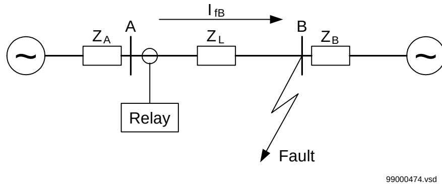
Figure 106: Through fault current from A to B: I_{fB}
